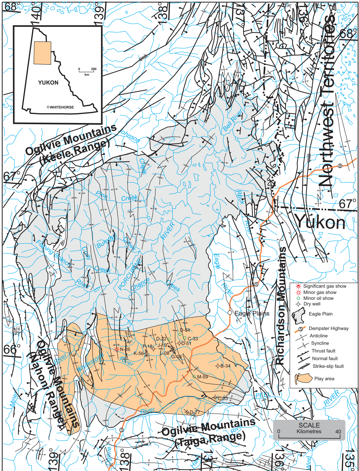
Figure 39. Canoe River carbonate structural oil and gas play.
