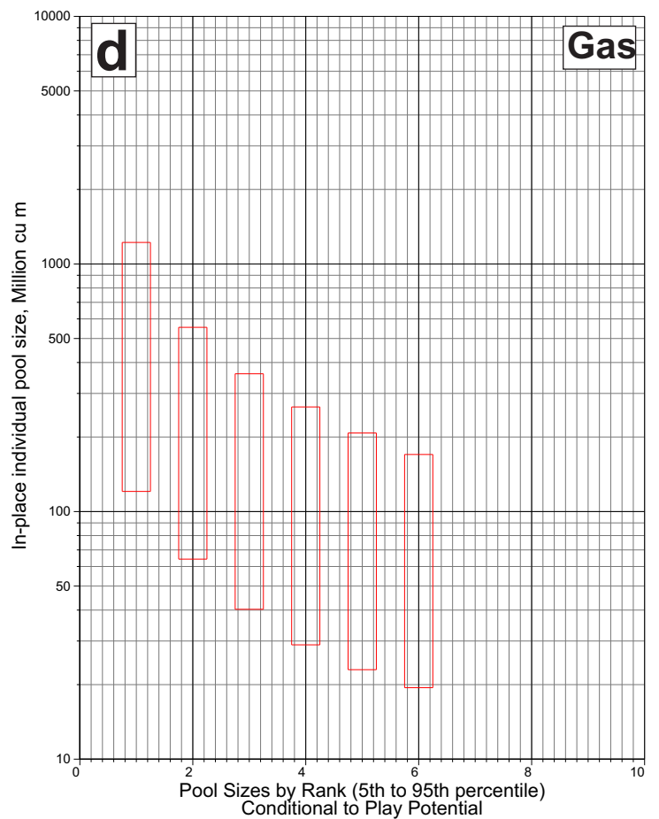
Figure 42. Estimates of in-place oil (a) and gas (c) potential of the Canoe River carbonate structural play. Pool-size-by-rank plots of the oil (b) and gas (d) plays are also displayed.
