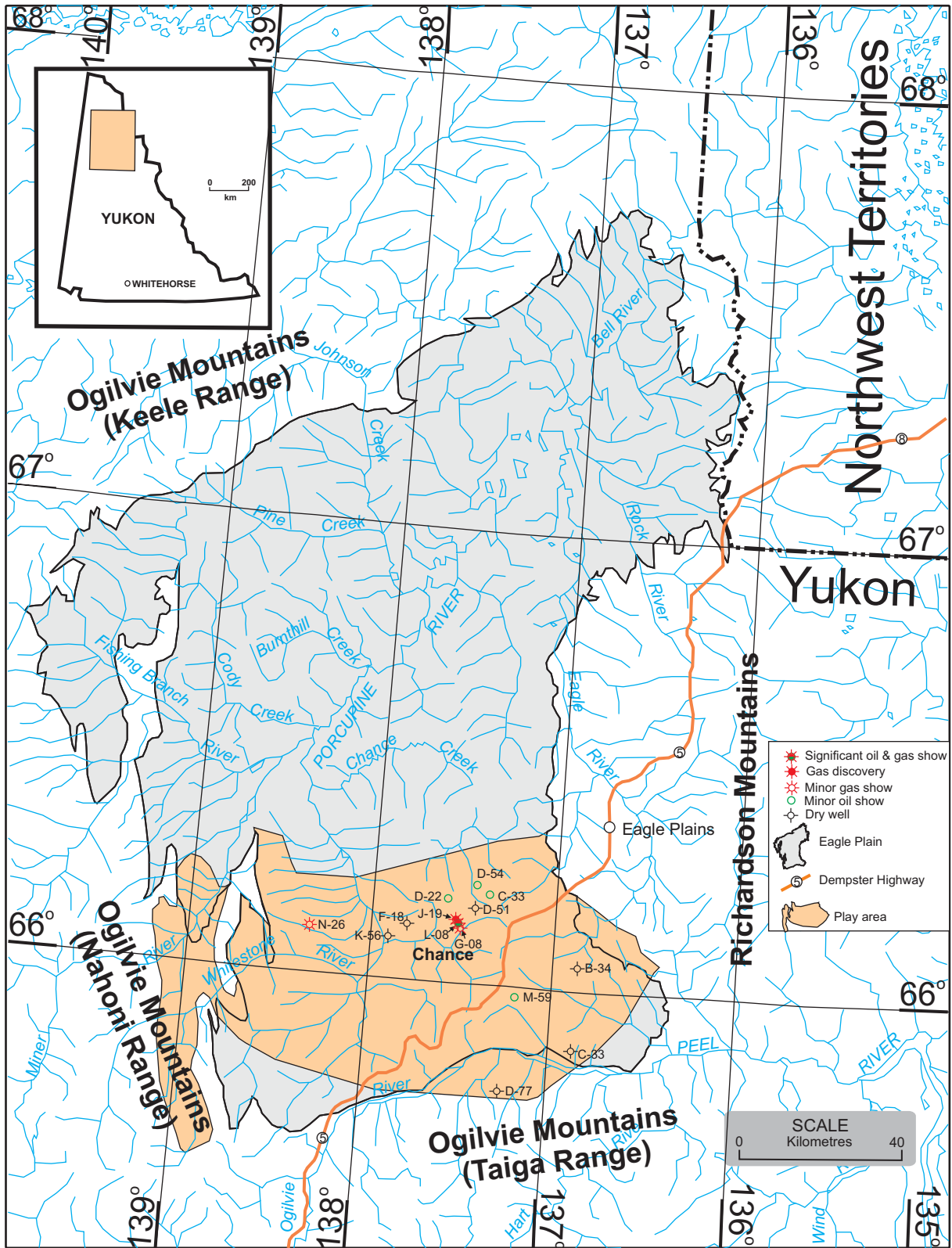
Figure 43. Canoe River carbonate stratigraphic oil and gas play.
