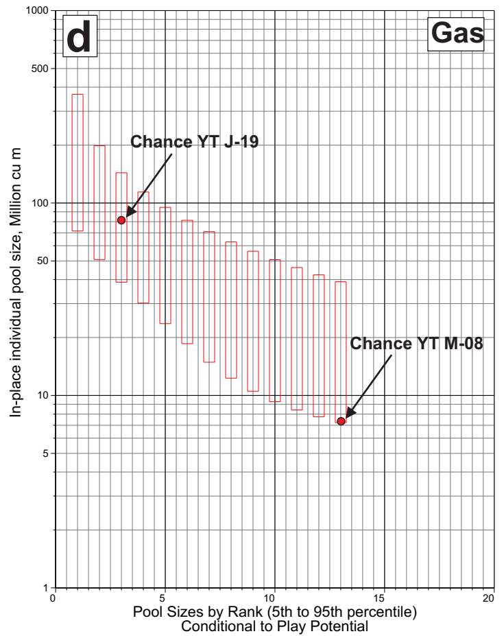
Figure 44. Estimates of in-place oil (a) and gas (c) potential of the Canoe River carbonate stratigraphic play. Pool-size-by-rank plots of the oil (b) and gas (d) plays are also displayed.
