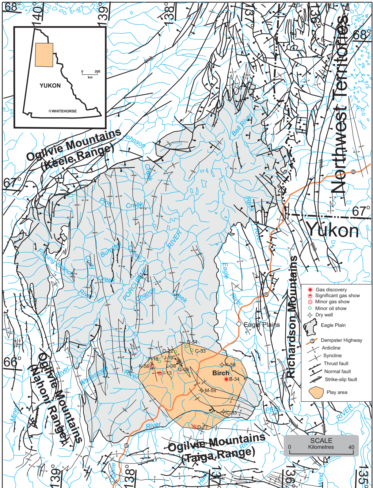
Figure 45. Chance sandstone structural oil and gas play.
