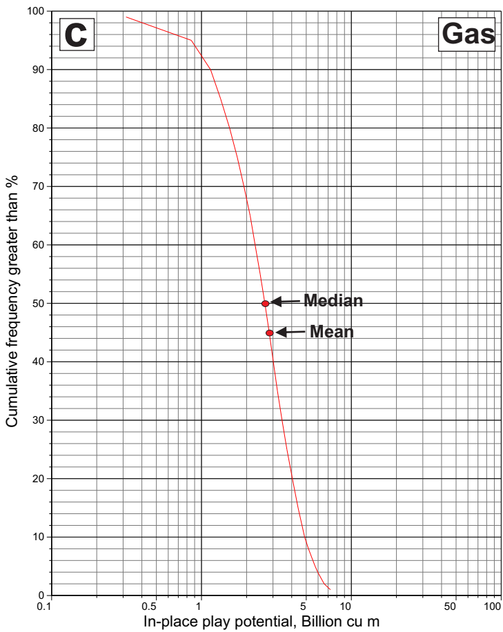
Figure 46. Estimates of in-place oil (a) and gas (c) potential of the Chance sandstone structural play. Pool-size-by-rank plots of the oil (b) and gas (d) plays are also displayed.
