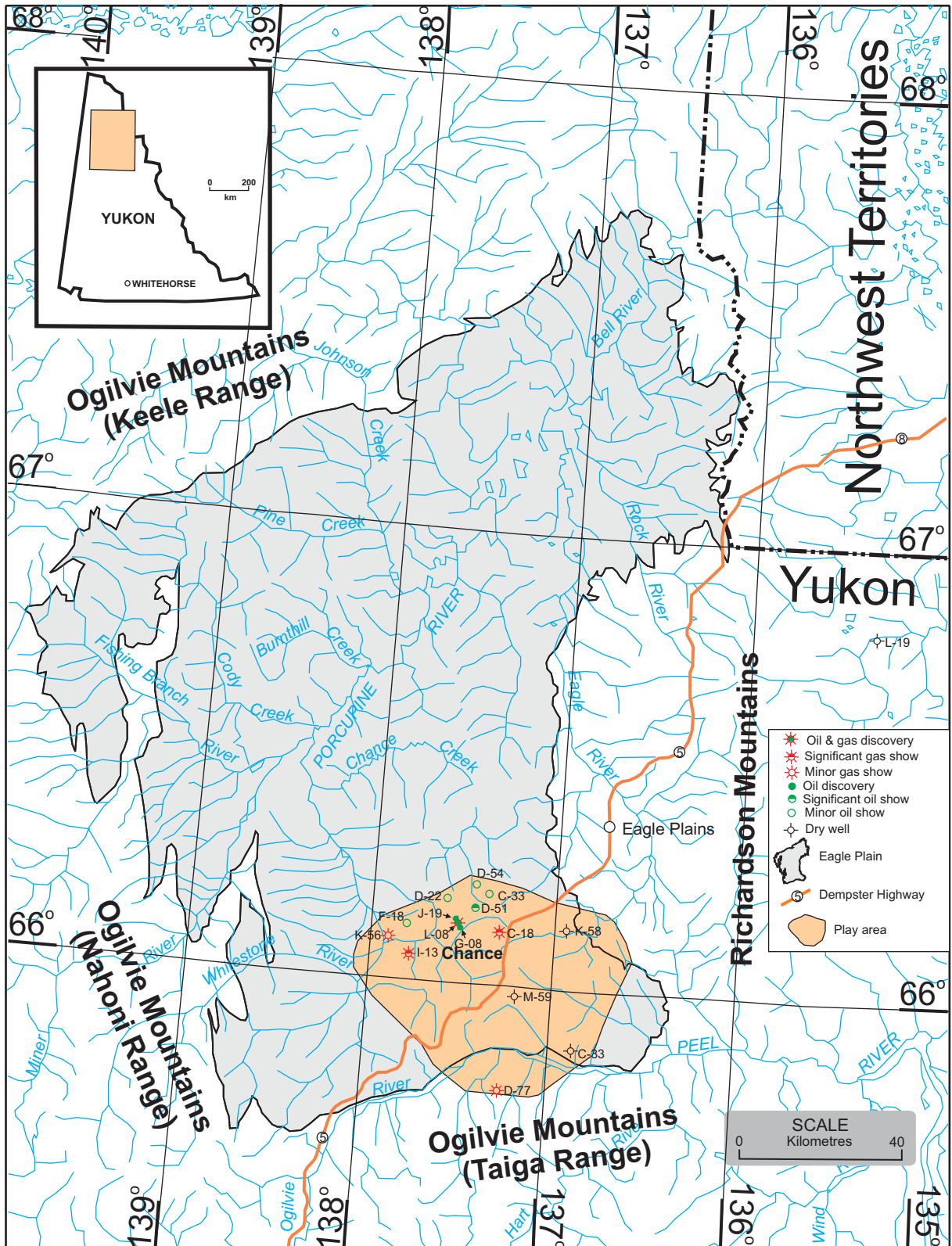
Figure 47. Chance sandstone stratigraphic oil and gas play.
