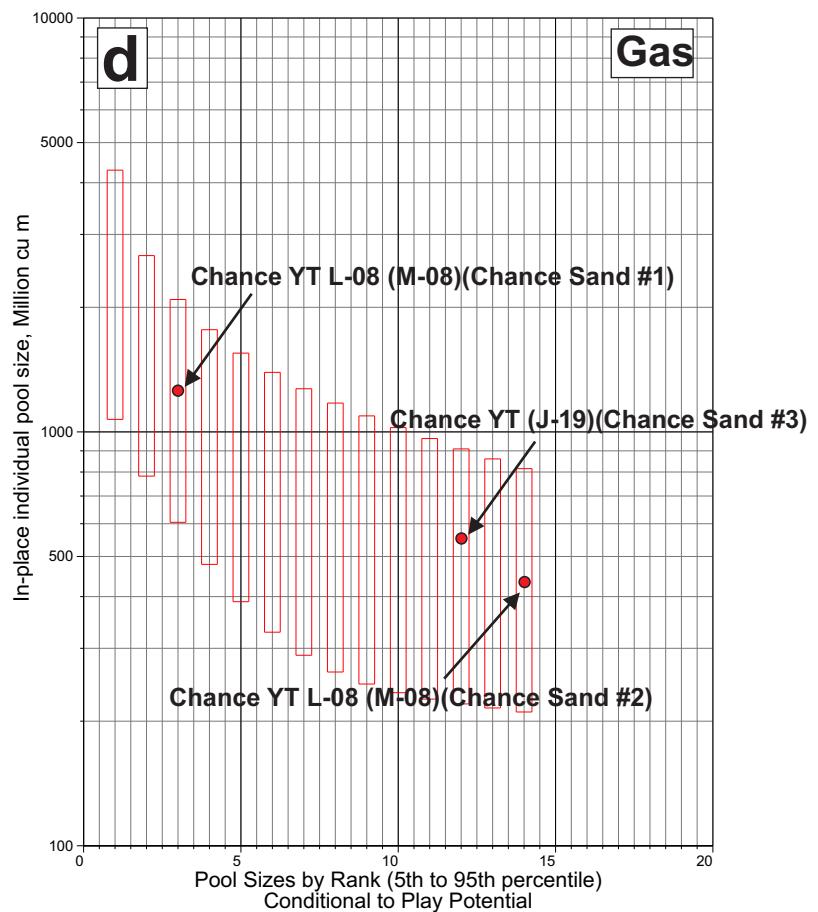
Figure 48. Estimates of in-place oil (a) and gas (c) potential of the Chance sandstone stratigraphic play. Pool-size-by-rank plots of the oil (b) and gas (d) plays are also displayed.
