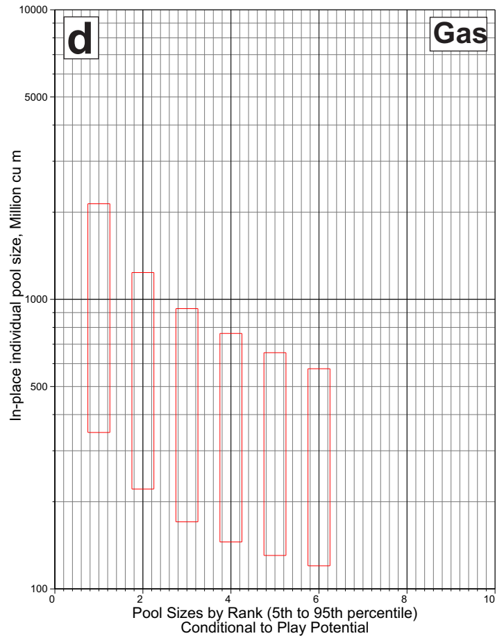
Figure 52. Estimates of in-place oil (a) and gas (c) potential of the Alder carbonate stratigraphic play. Pool-size-by-rank plots of the oil (b) and gas (d) plays are also displayed.
