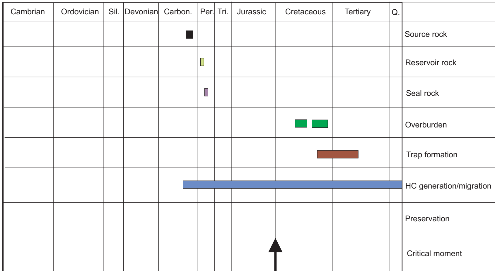
Figure 56. Petroleum event chart for a Carboniferous-Permian petroleum system (Blackie source-Jungle Creek reservoir). The critical moment for oil and gas generation (arrow) in southern Eagle Plain occurred during Late Jurassic/Early Cretaceous time, the midway point of thermal oil and gas generation derived from the burial history diagrams of Link and Bustin (1989). Sil.-Silurian, Carbon.-Carboniferous, Per.-Permian, Tri.-Triassic, Q.-Quaternary.
