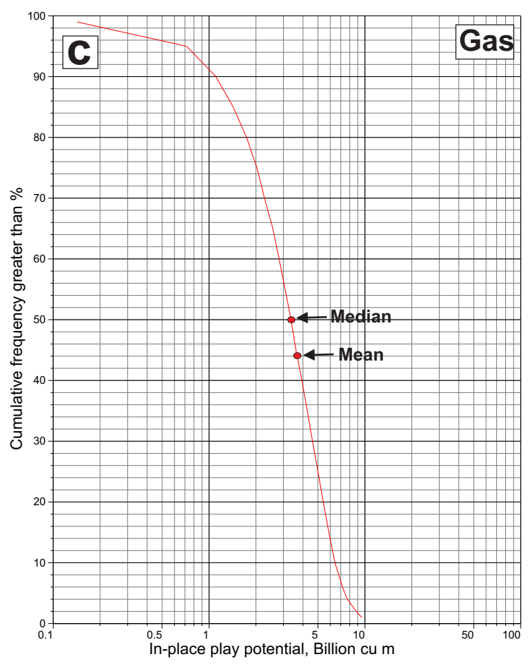
Figure 57. Estimates of in-place oil (a) and gas (c) potential of the Jungle Creek sandstone structural play. Pool-size-by-rank plots of the oil (b) and gas (d) plays are also displayed.
