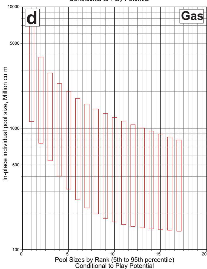
Figure 59. Estimates of in-place oil (a) and gas (c) potential of the Jungle Creek sandstone stratigraphic play. Pool-size-by-rank plots of the oil (b) and gas (d) plays are also displayed.
