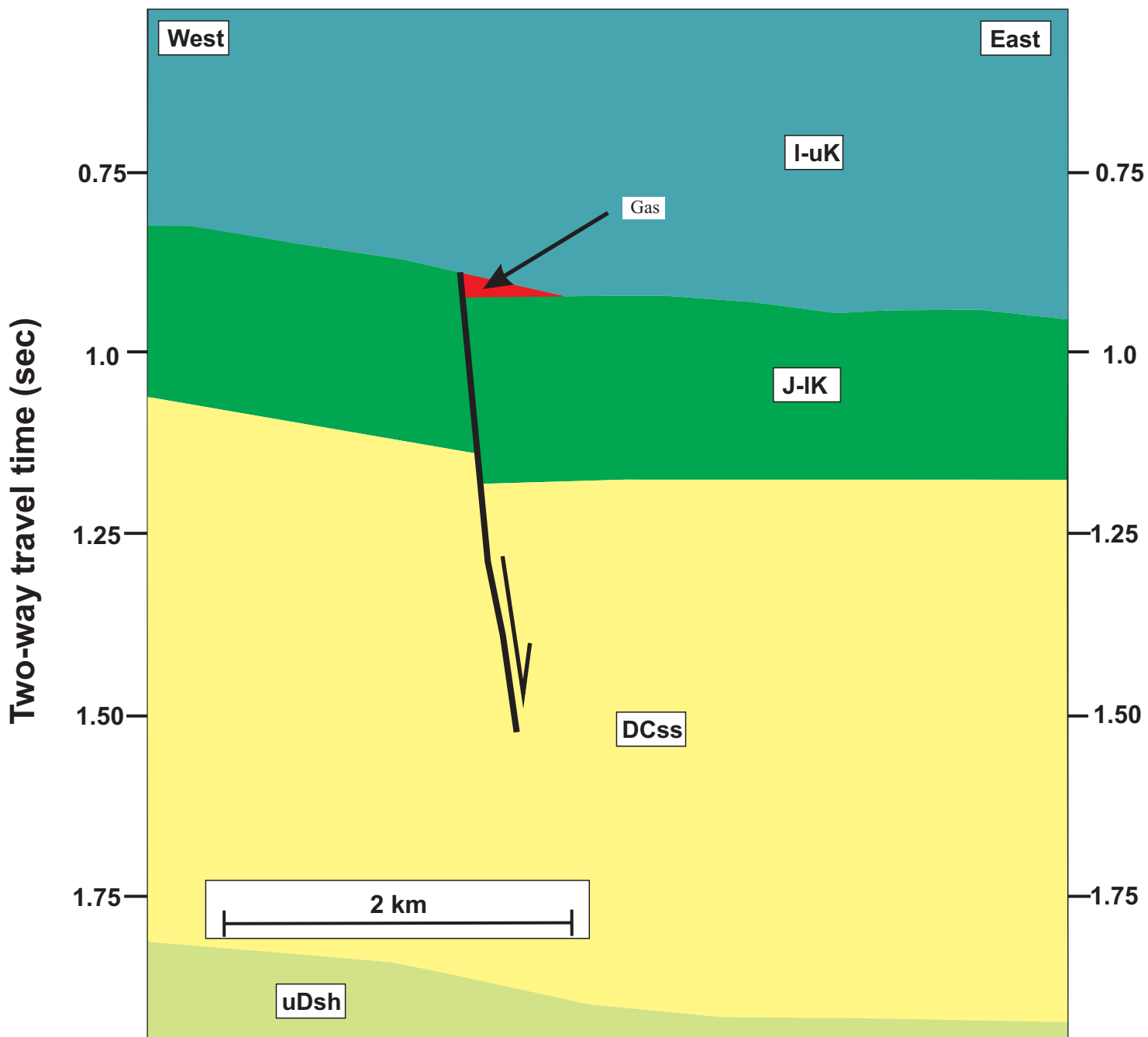
Figure 62. Schematic seismic section illustrating a pre-Albian normal fault structure and potential trap configuration in Sharp Mountain Subbasin (see Fig. 60 for location). Local preservation of hanging-wall strata within interbedded sandstone and shale succession (Jurassic-Lower Cretaceous; J-IK). From Lane (2010). Part of Chevron Canada Resources seismic reflection line 12bb. I-uK, Lower to Upper Cretaceous clastic succession; J-IK, Jurassic to Lower Cretaceous clastic succession; DCss, Imperial/Tuttle formations; Dsh, Upper Devonian Imperial Formation, shale dominant succession.
