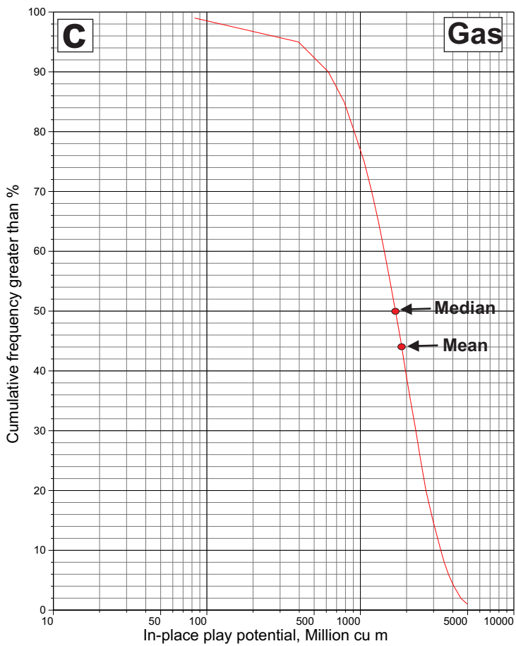
Figure 63. Estimates of in-place oil (a) and gas (c) potential of the Jurassic-Lower Cretaceous sandstone pre-Albian structural play. Pool-size-by-rank plots of the oil (b) and gas (d) plays are also displayed.
