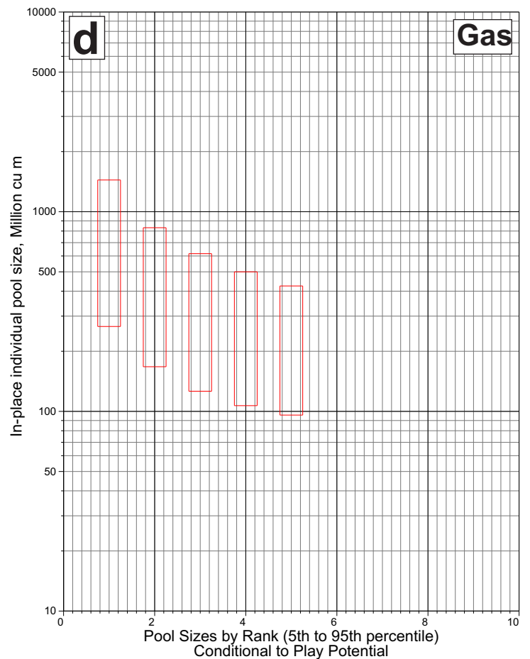
Figure 63. Estimates of in-place oil (a) and gas (c) potential of the Jurassic-Lower Cretaceous sandstone pre-Albian structural play. Pool-size-by-rank plots of the oil (b) and gas (d) plays are also displayed.
