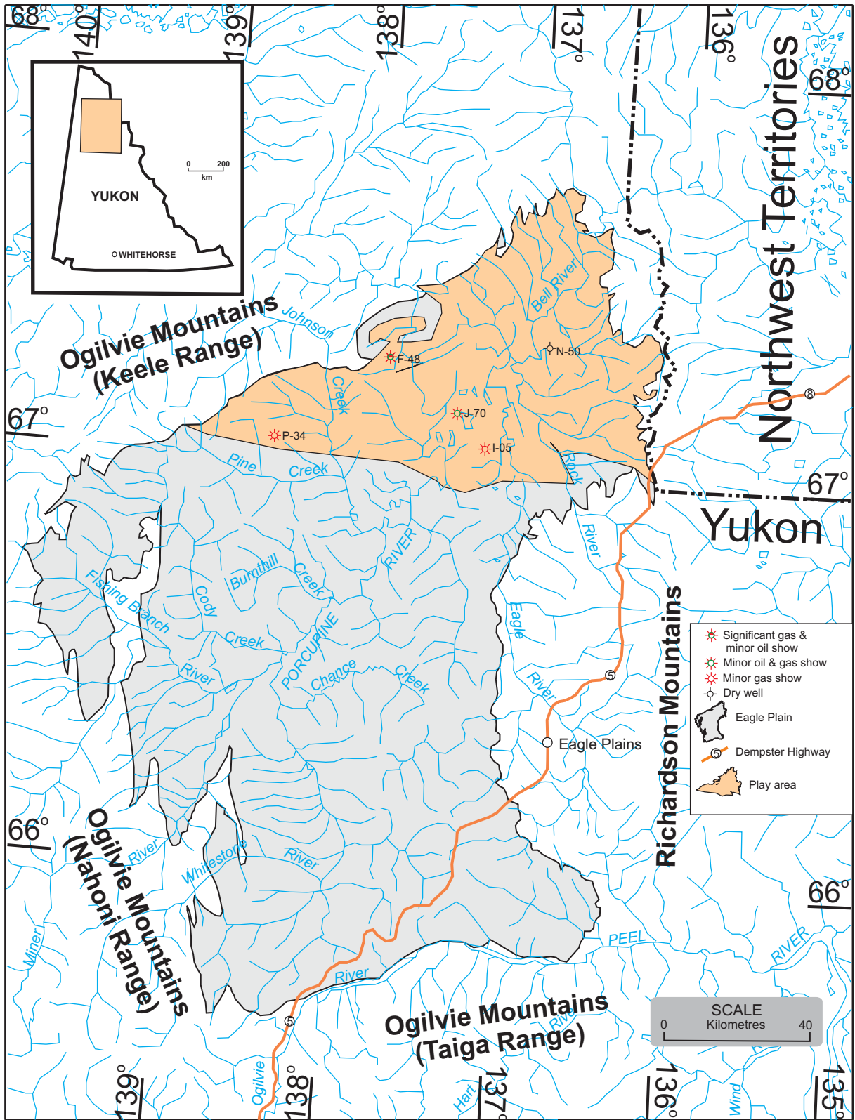
Figure 64. Jurassic/Lower Cretaceous sandstone stratigraphic oil and gas play.
