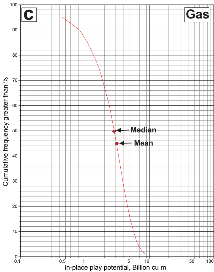
Figure 65. Estimates of in-place oil (a) and gas (c) potential of the Jurassic-Lower Cretaceous sandstone stratigraphic play. Pool-size-by-rank plots of the oil (b) and gas (d) plays are also displayed.
