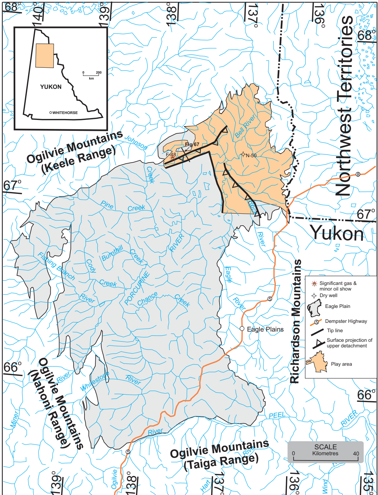
Figure 66. Triangle zone structural (Bell Subbasin) oil and gas play. Tip lines and upper detachment projections of triangle zones are from Lane (1996). Seismic line location of Fig. 67 is shown.
