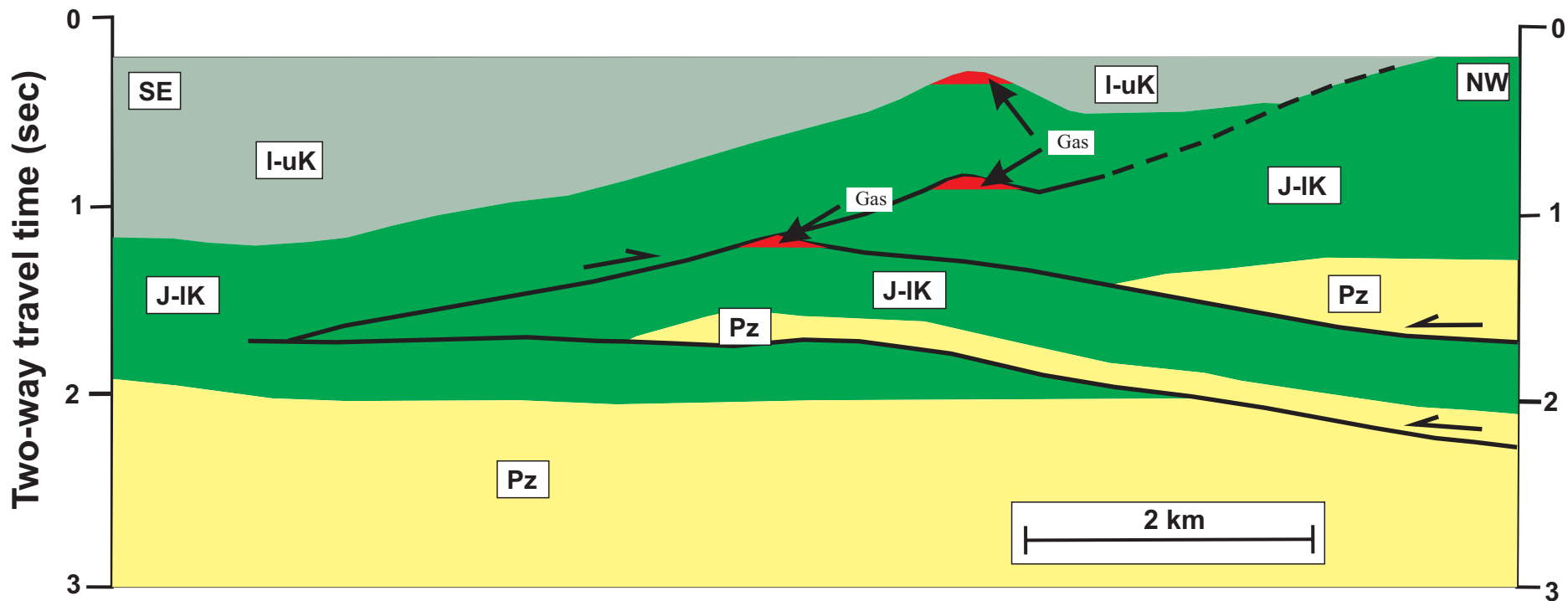
Figure 67. Schematic seismic section illustrating thrust-repeated stacked reservoirs, fault-propagation folds and subthrust structures associated with backthrusts in a triangle zone adjacent to Dave Lord Mountains in the Keele Range (see Fig. 66 for location). From Lane (1996). Chevron Canada Resources seismic reflection line 39X. I-uK, Lower to Upper Cretaceous clastic succession; J-IK, Jurassic to Lower Cretaceous clastic succession; Pz, Paleozoic succession. Faults are dashed when inferred.
