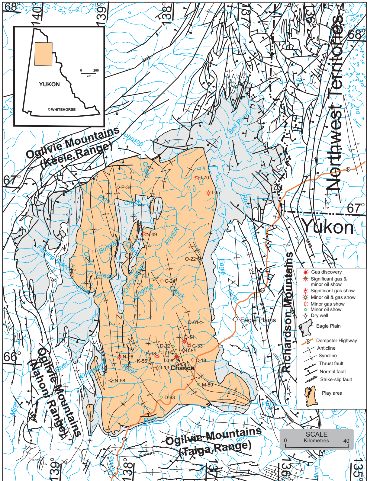
Figure 69. Cretaceous sandstone structural oil and gas play.
