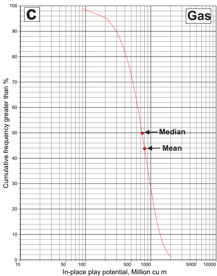
Figure 73. Estimates of in-place oil (a) and gas (c) potential of the Cretaceous sandstone shelf stratigraphic play. Pool-size-by-rank plots of the oil (b) and gas (d) plays are also displayed.
