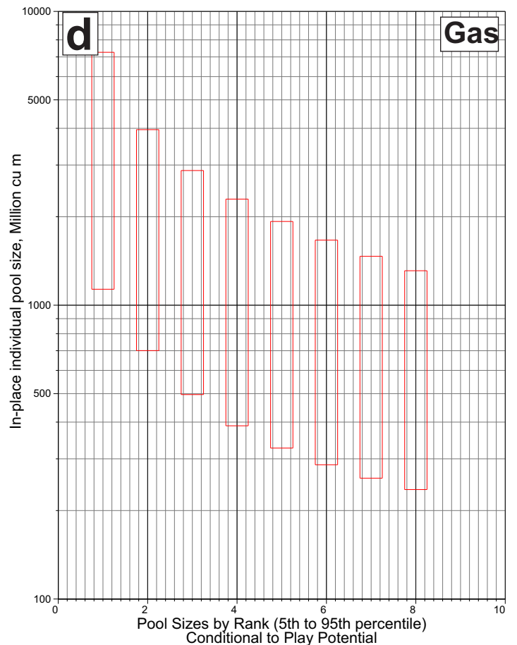
Figure 75. Estimates of in-place oil (a) and gas (c) potential of the Cretaceous sandstone slope stratigraphic play. Pool-size-by-rank plots of the oil (b) and gas (d) plays are also displayed.
