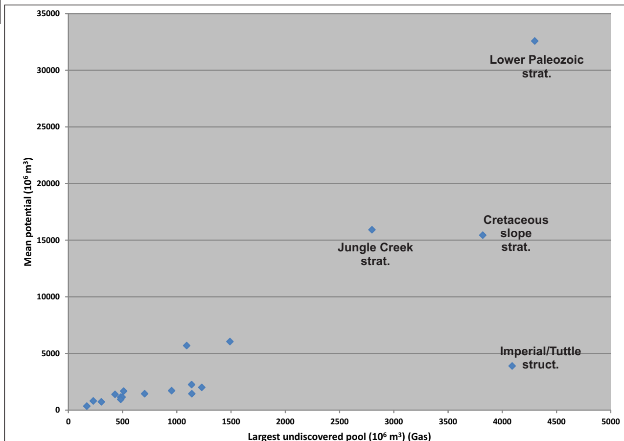
Figure 78. Plots showing the relation of mean play potential to undiscovered pool sizes of all oil plays (a) and all gas plays (b) in Eagle Plain Basin.
