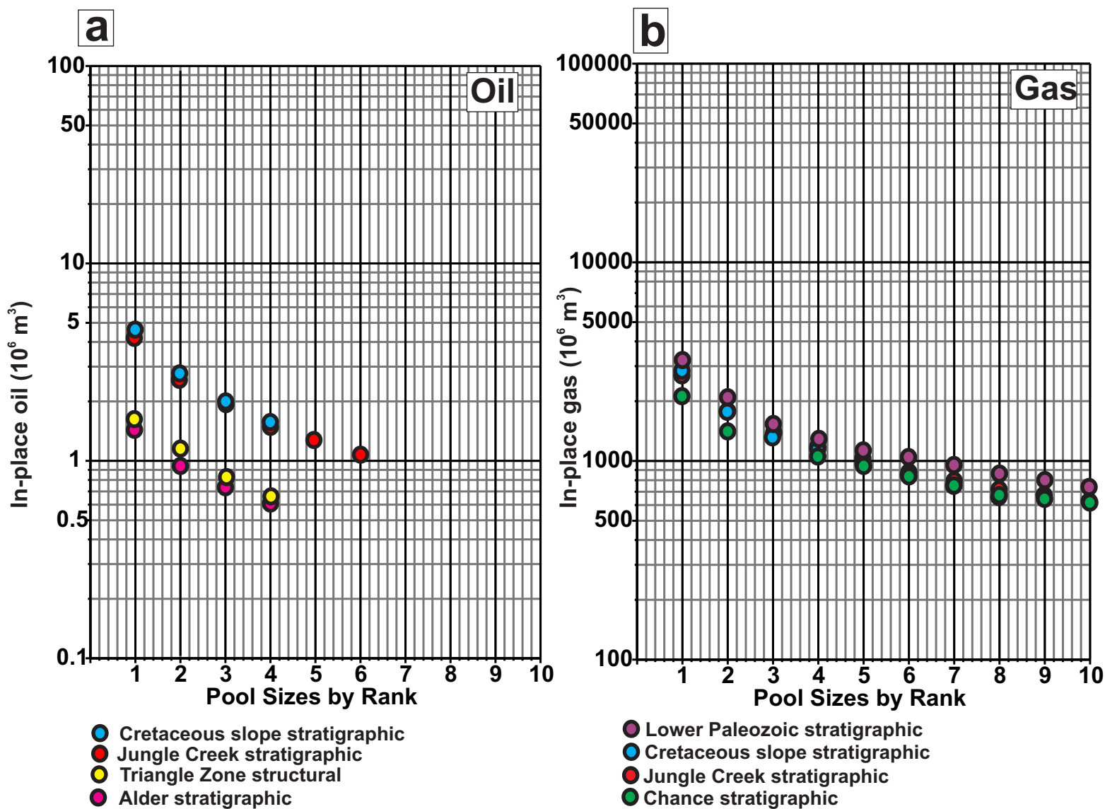
Figure 79. Pool-size-by-rank plots of largest undiscovered oil (a) and gas (b) pools showing relationships between significant plays, Eagle Plain Basin. Median pool sizes are plotted.
