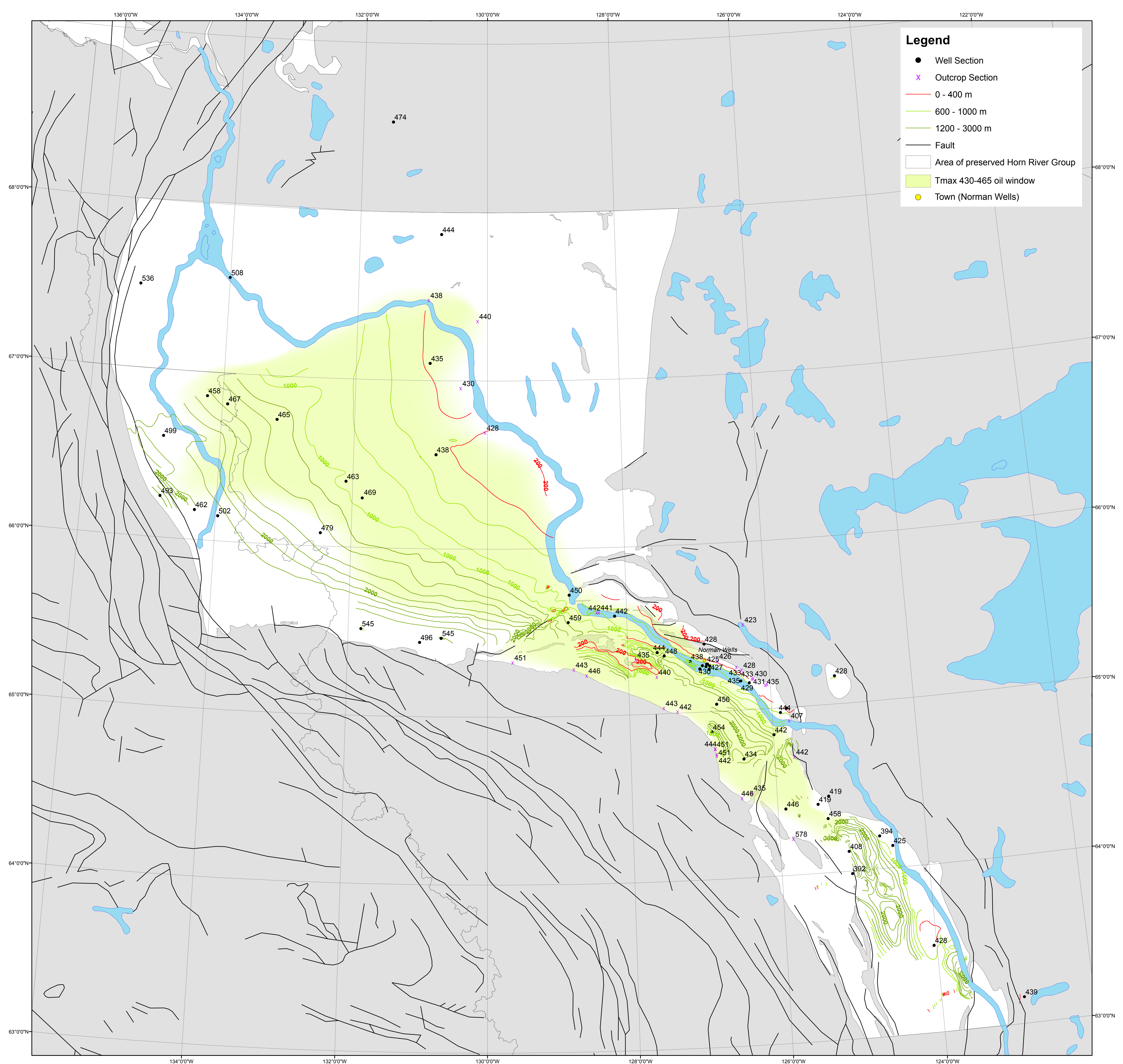
Combined depth and thermal maturity map of the Canol Formation, northern Mackenzie Valley, NWT
