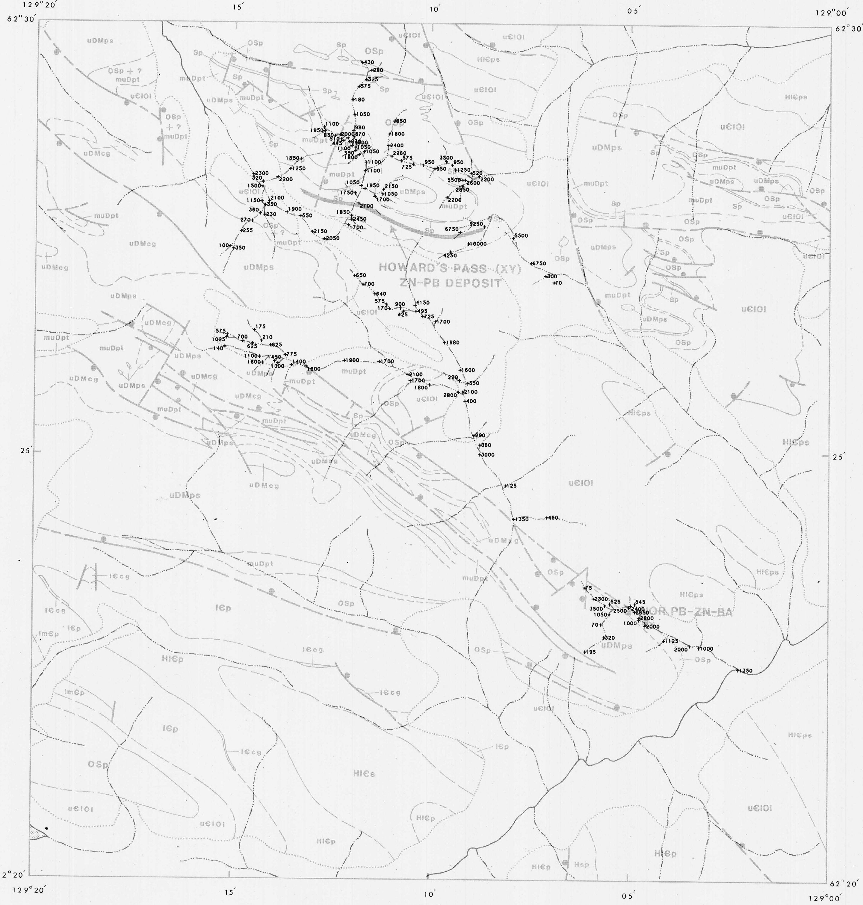
ZINC Parts per million in stream sediments
