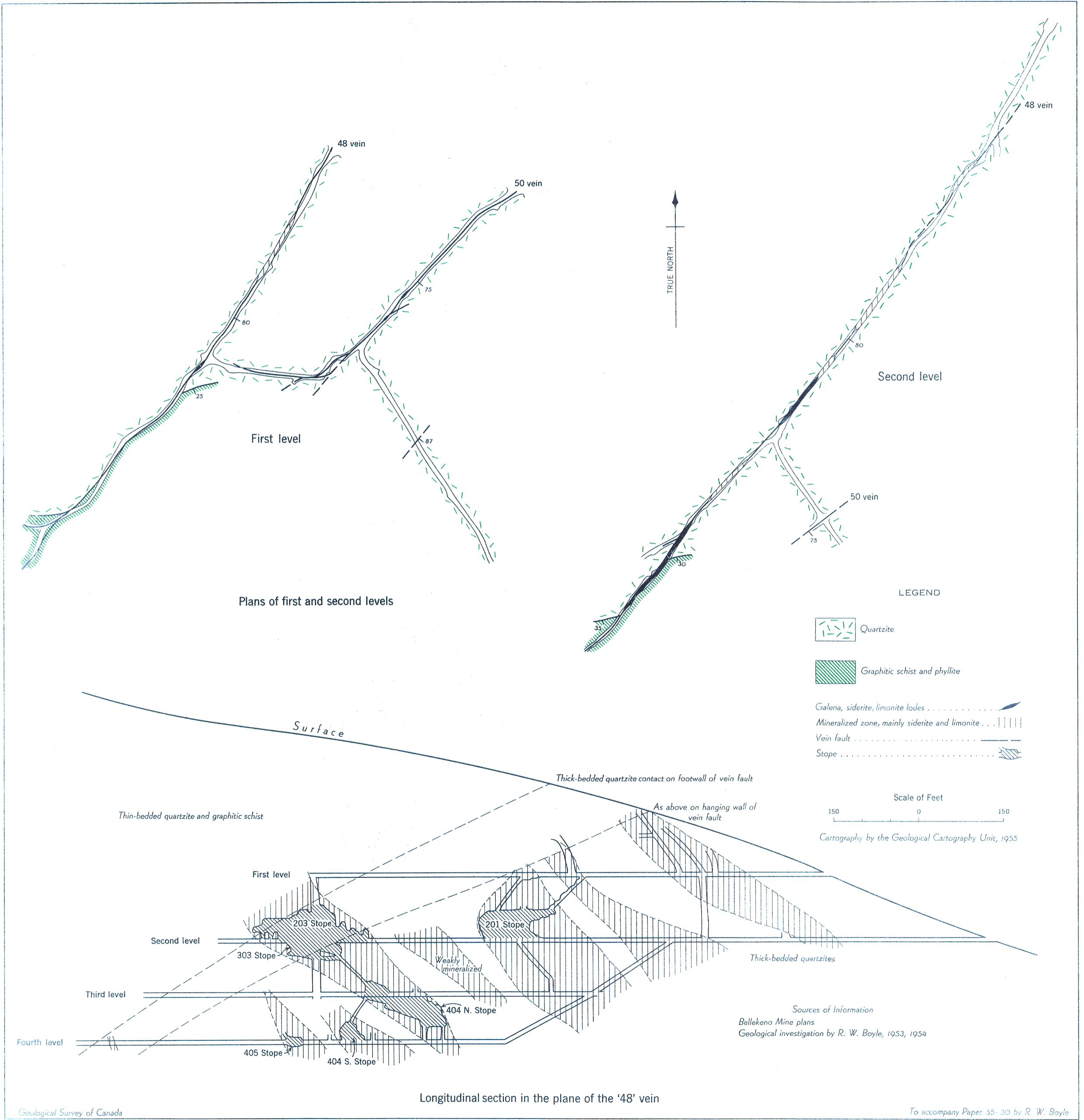
Figure 9. Plans and longitudinal section, Bellekeno Mine, Sourdough Hill, Yukon Territory
