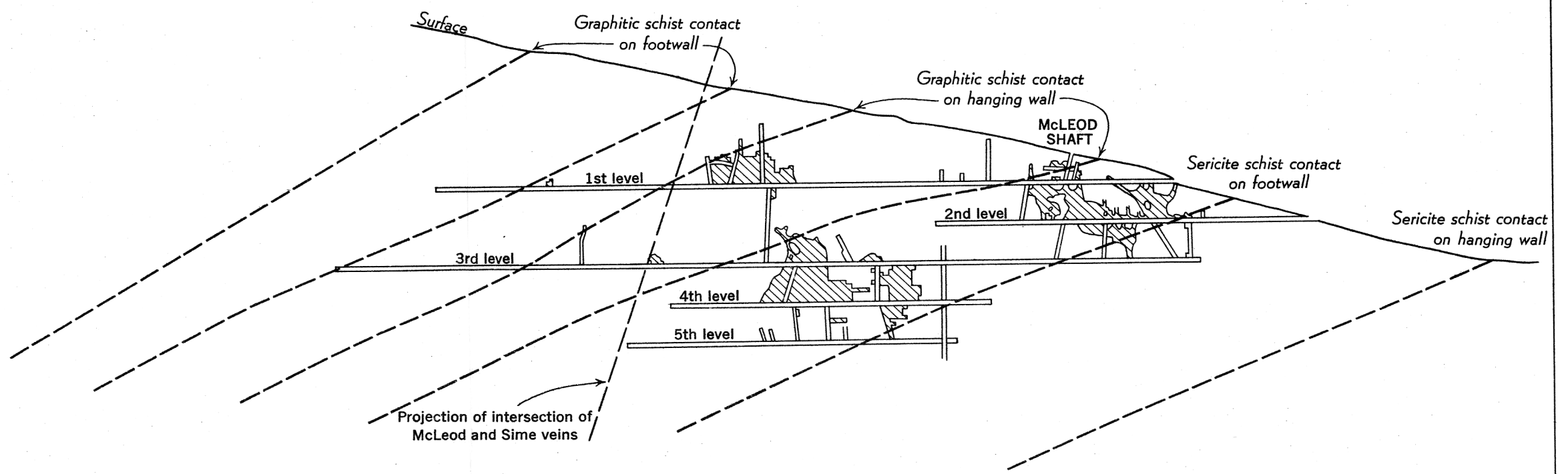
Longitudinal section in the plane of the McLeod vein
