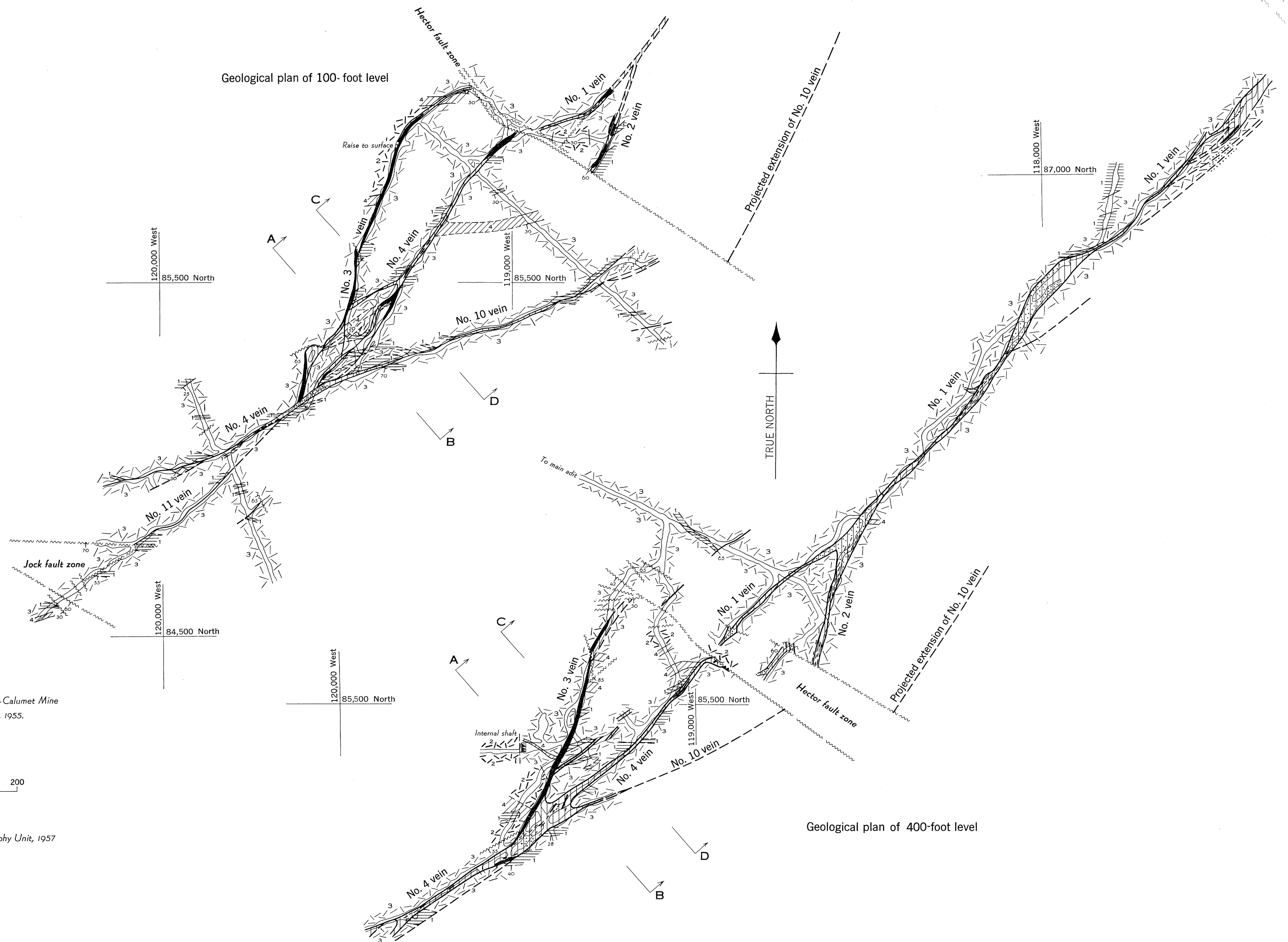
Figure 3. Geological plans and sections, Hector-Calumet Mine, Galena Hill, Yukon Territory
