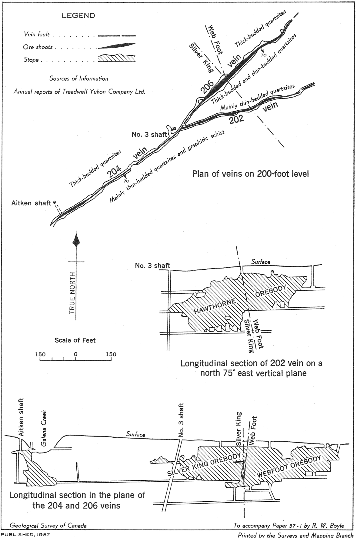
Figure 5. Plan and longitudinal sections, Silver King Mine, Galena Hill, Yukon Territory
