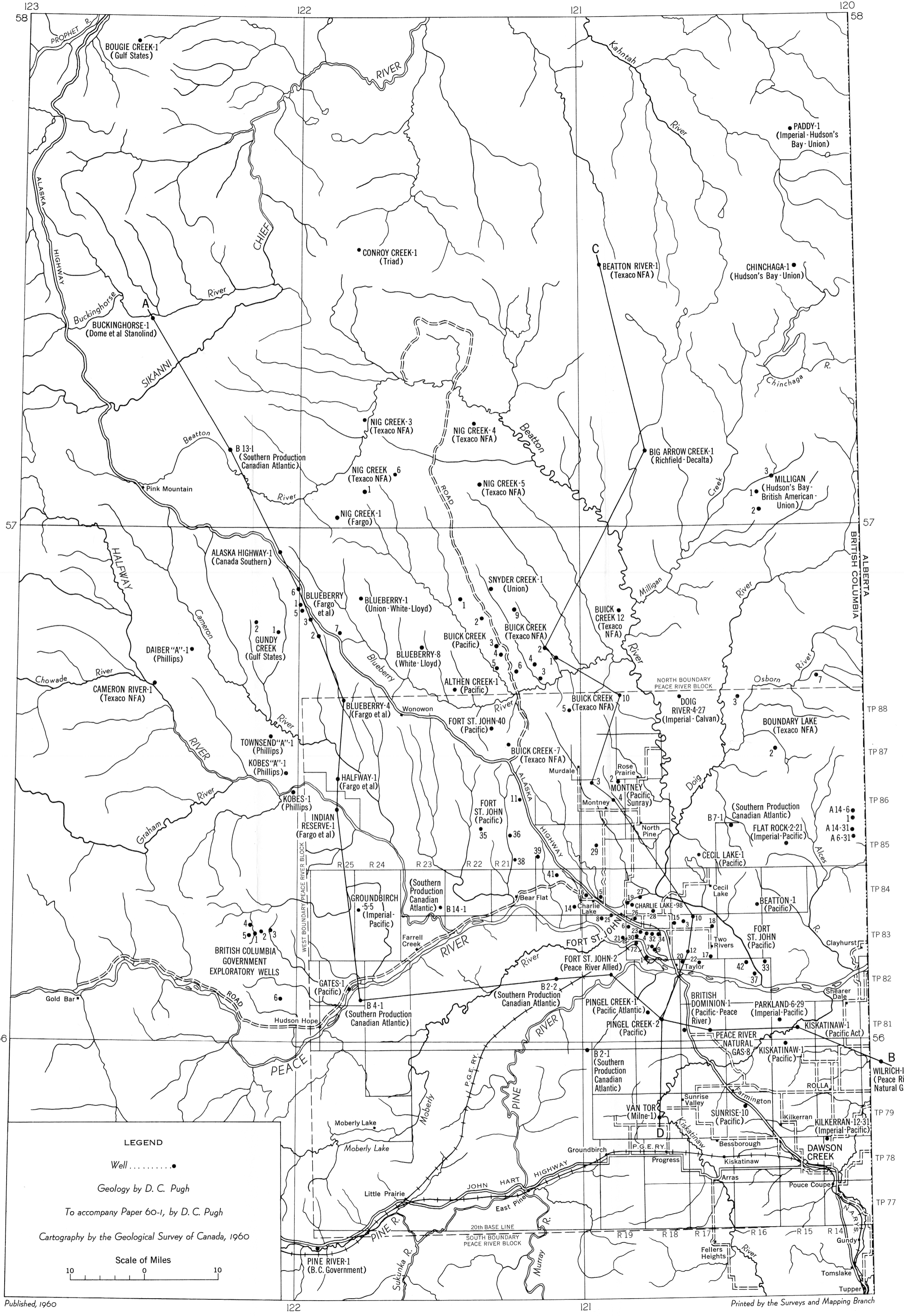
Figure 1. Index map, Fort St. John area, Peace River District, British Columbia, showing location and identity of wells from which information has been used, and lines of stratigraphic sections (A-B, C-D) illustrated in Figures 5 and 6
