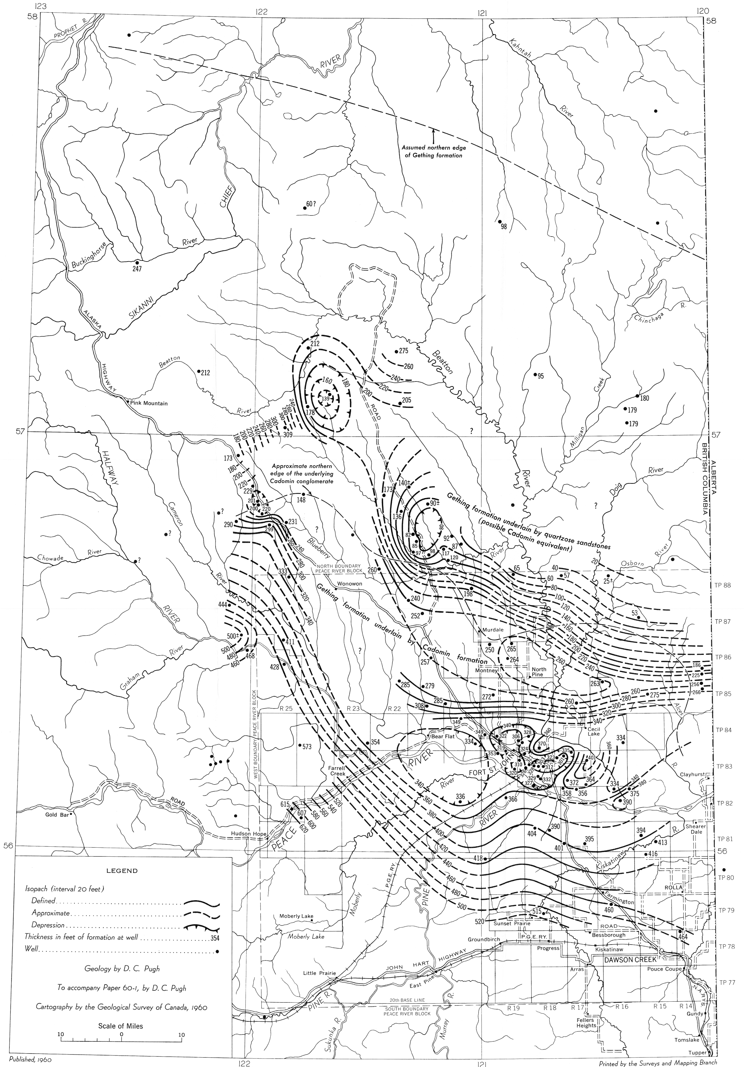
Figure 2. Map of Fort St. John area, Peace River District, British Columbia, showing isopachs of the Gething formation
