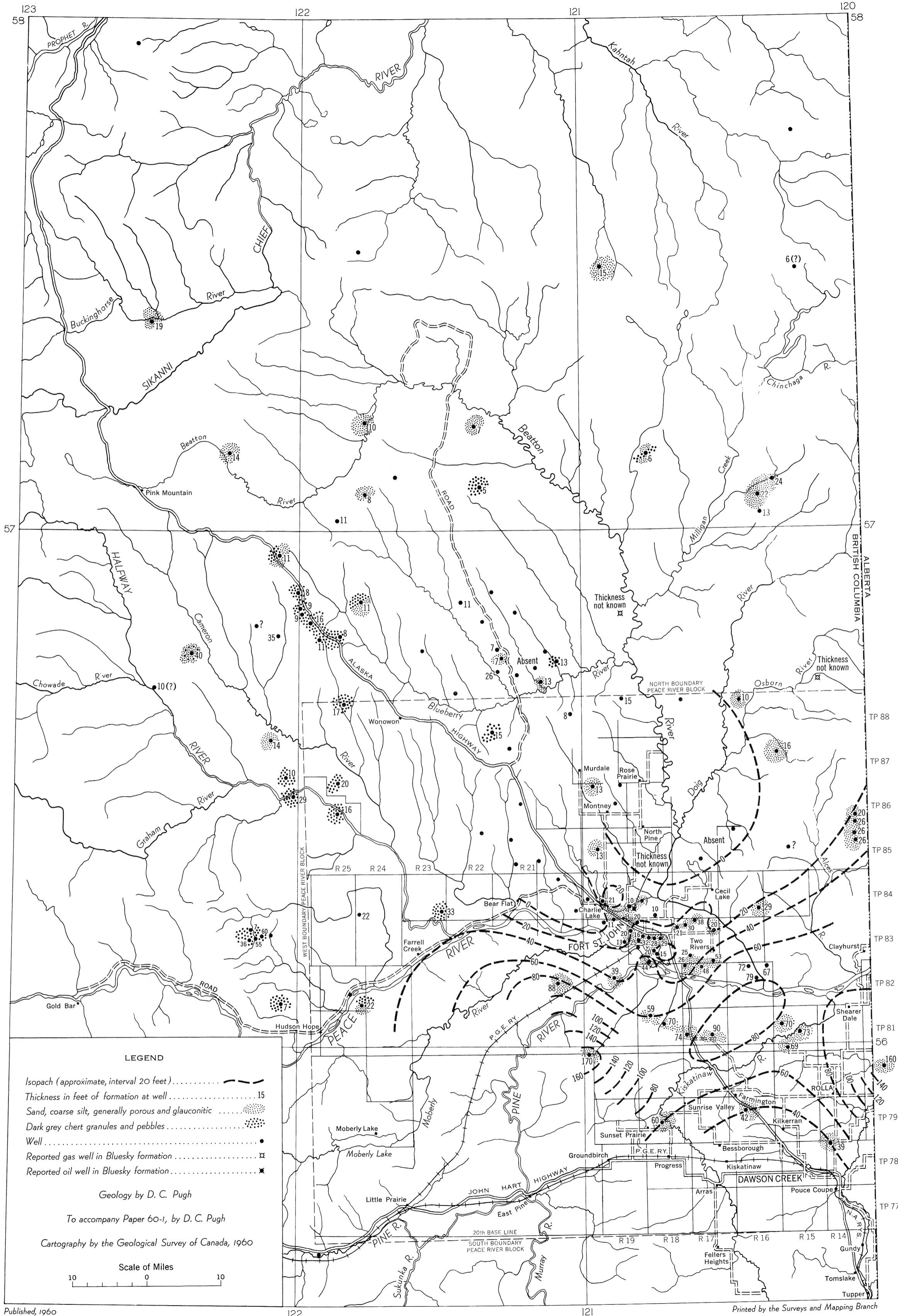
Figure 3. Map of Fort St. John area, Peace River District, British Columbia, showing isopachs, lithology, and distribution of Bluesky formation
