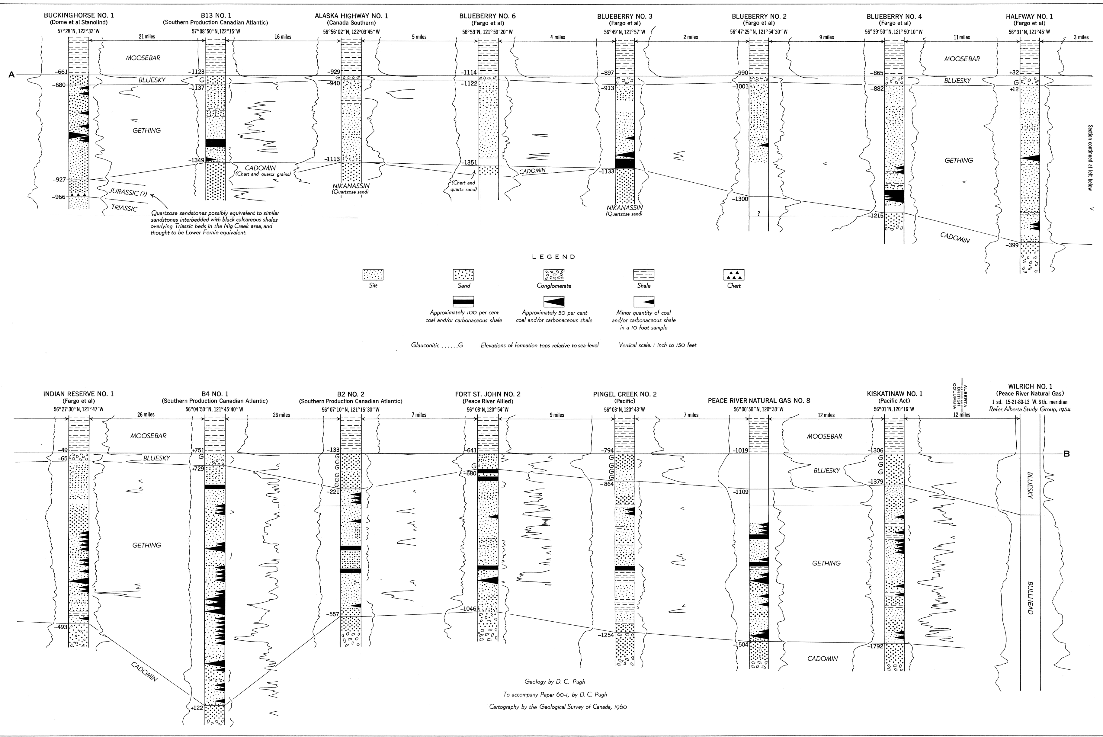
Figure 5. Stratigraphic section on line A-B (Figure 1), Peace River District, British Columbia
