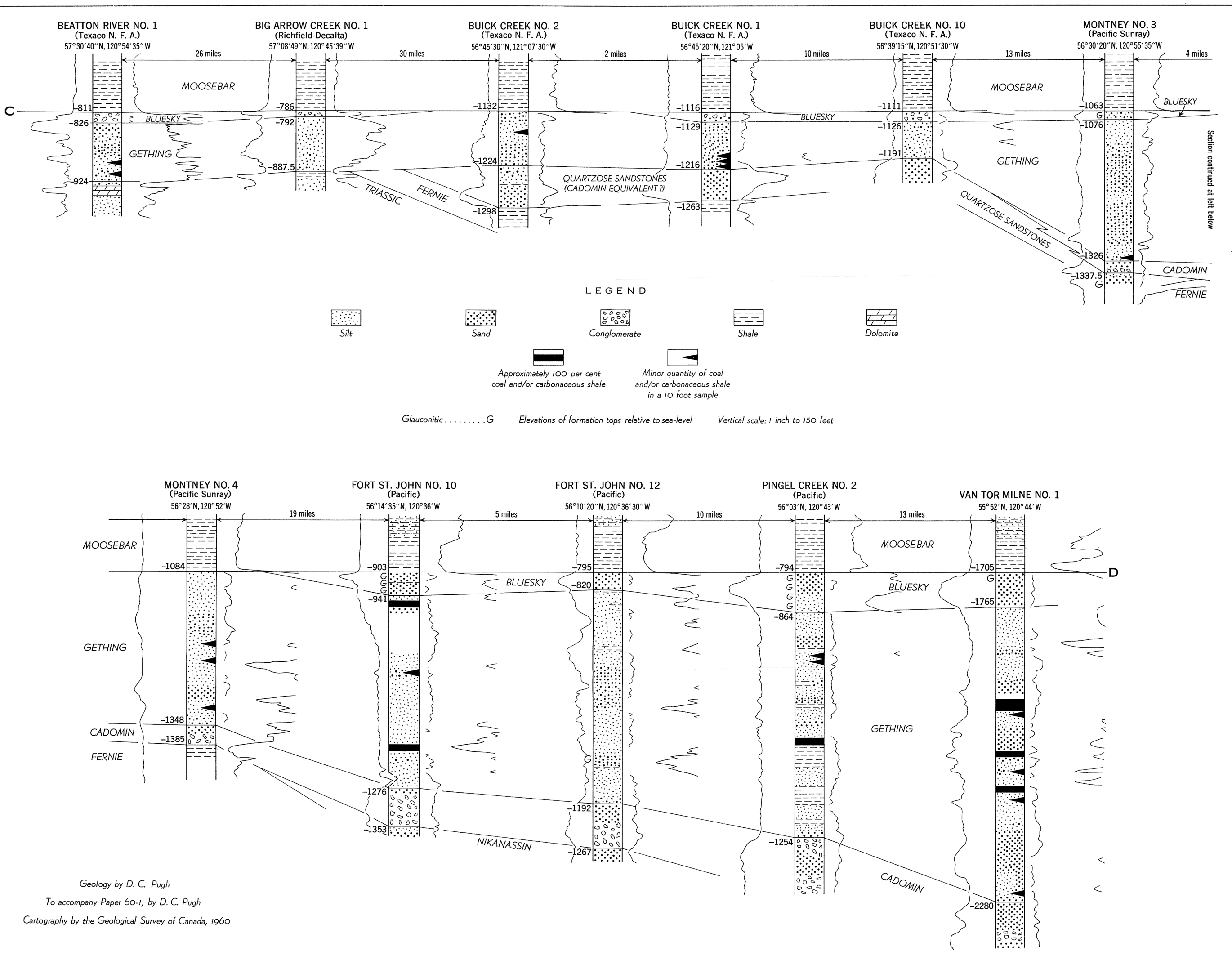
Figure 6. Stratigraphic section on line C-D (Figure 1), Peace River District, British Columbia
