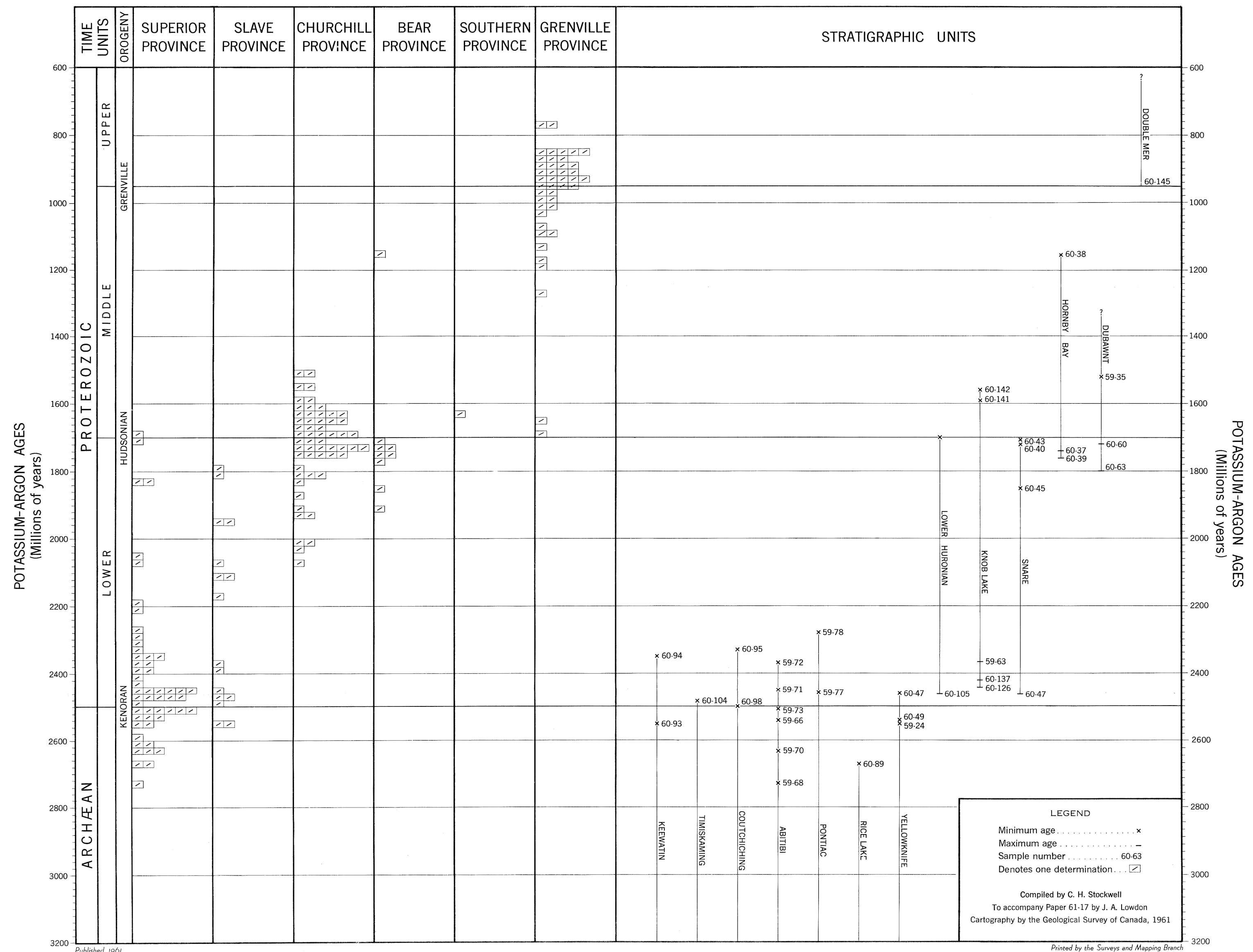
Figure 6. Potassium-Argon ages in the Canadian Shield
