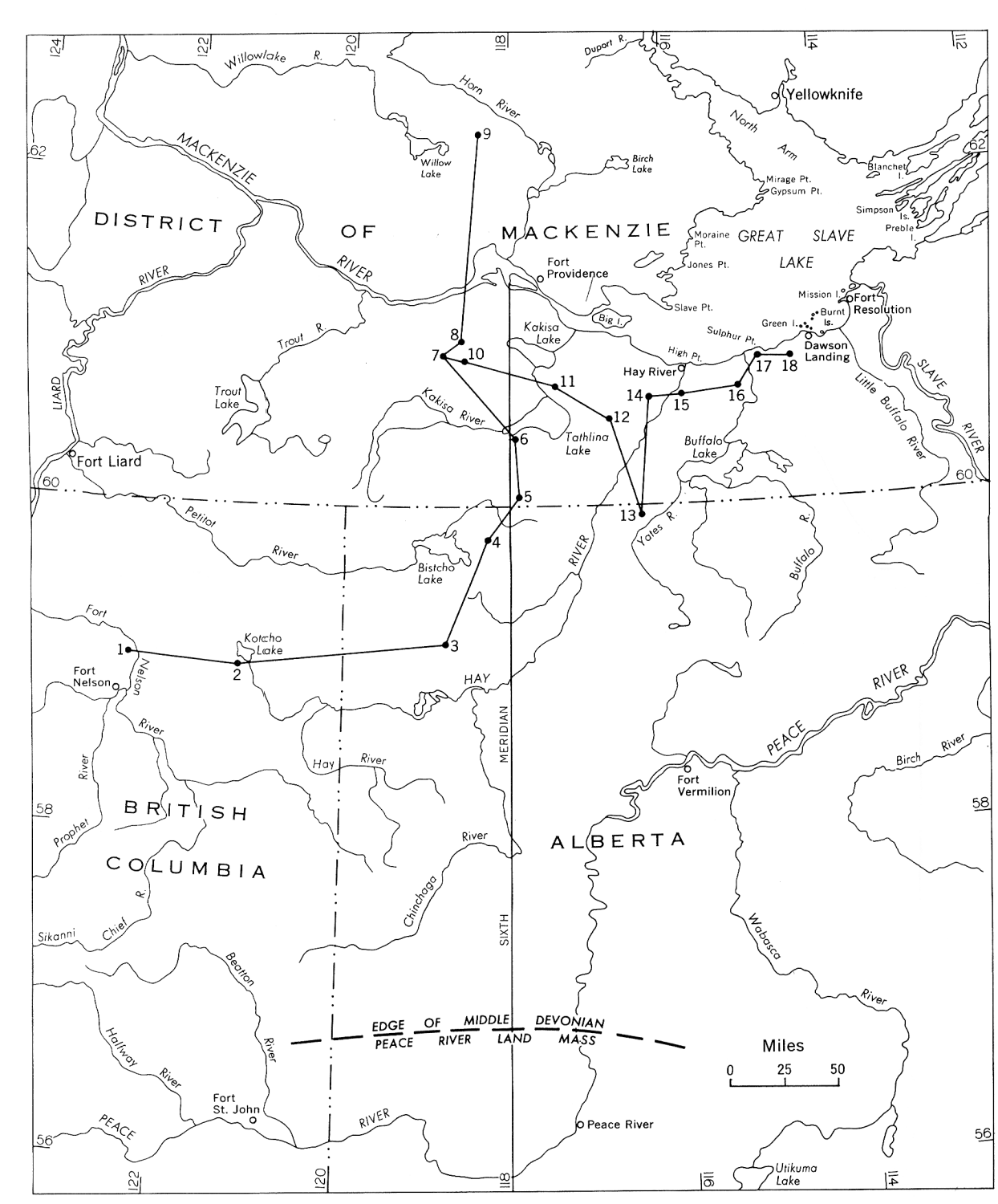
Index map showing locations of sections
