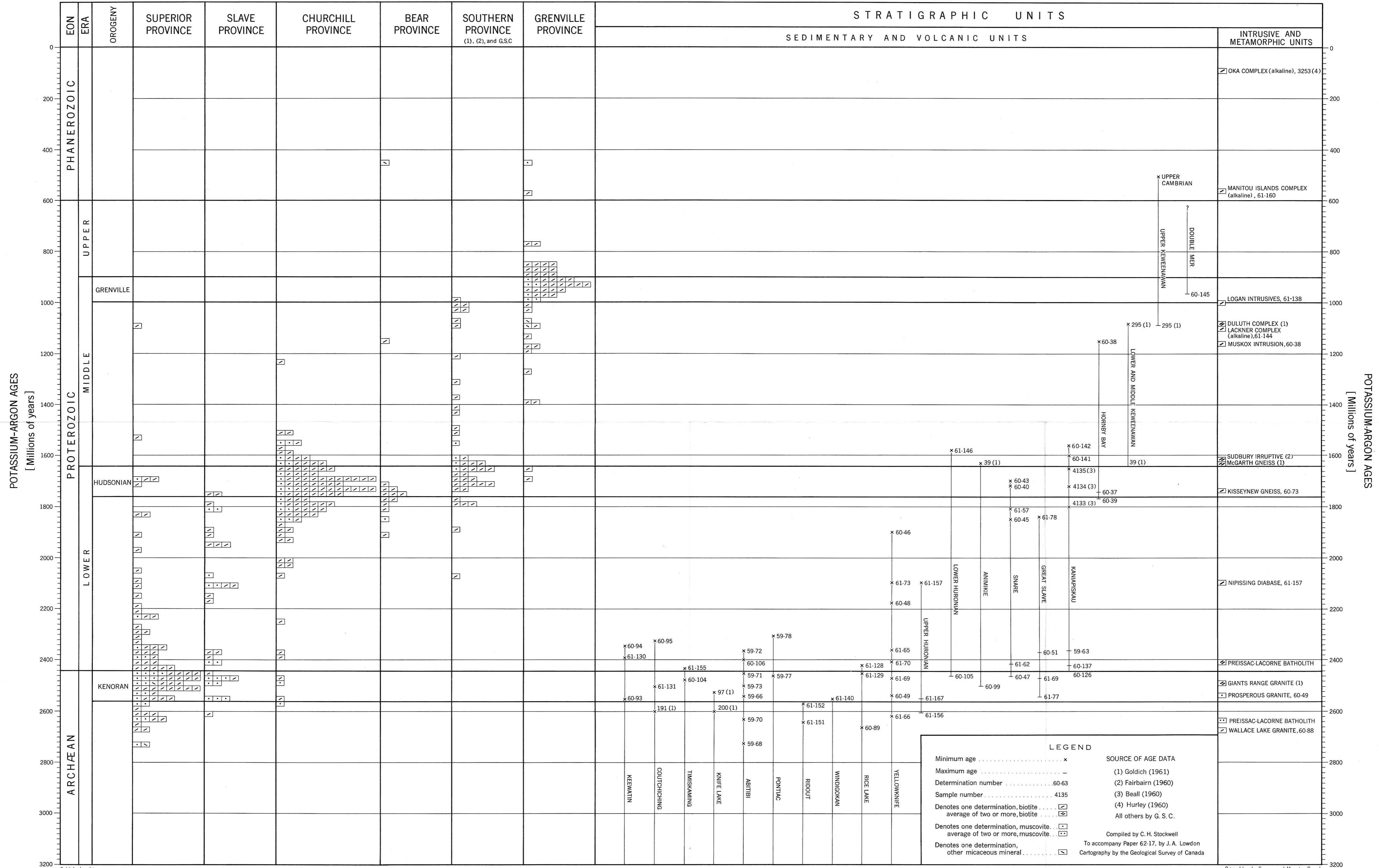
Figure 3. Potassium-Argon ages on micas of the Canadian Shield
