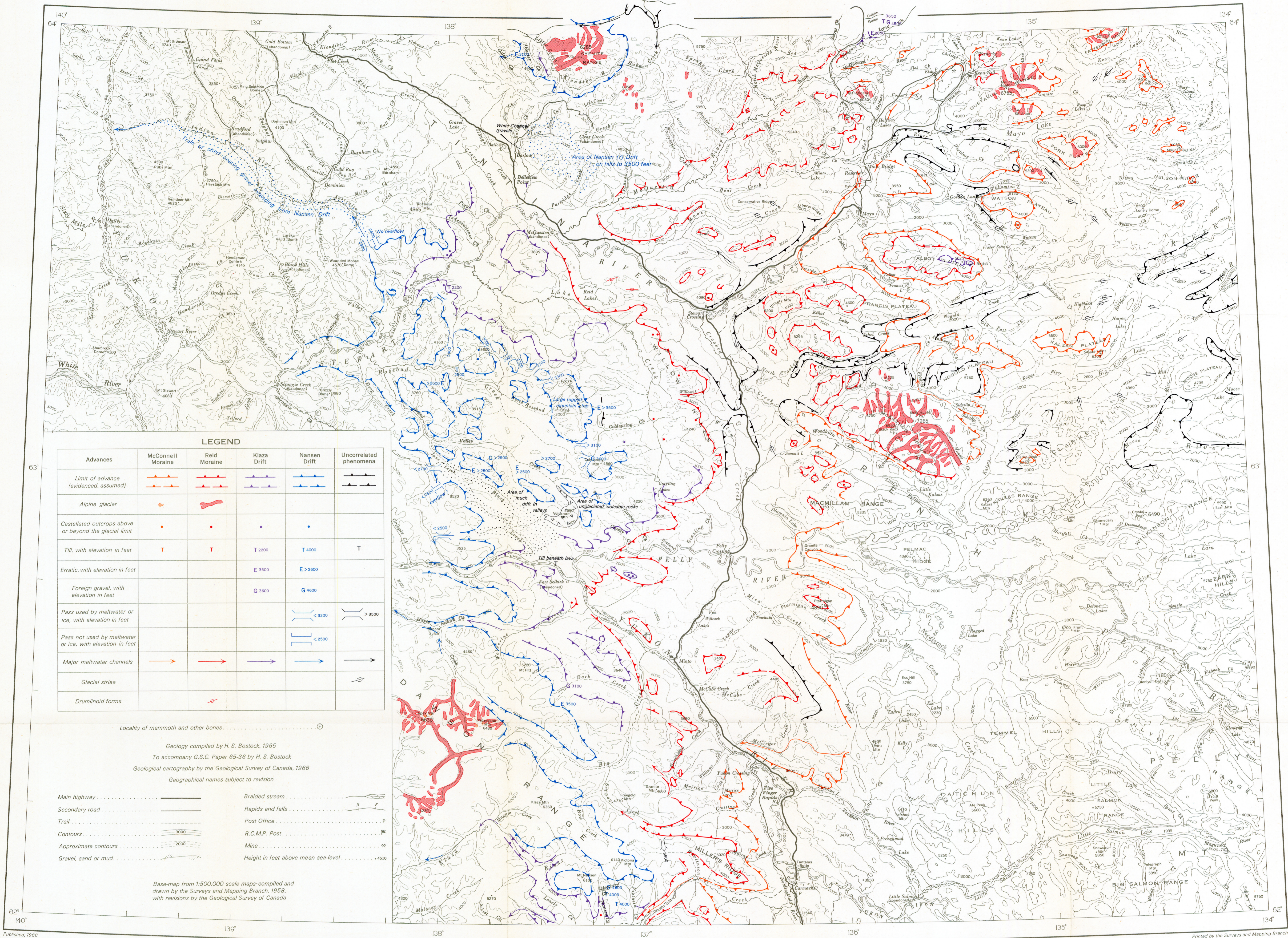
Figure 1. Glacial geology of part of central Yukon Territory
