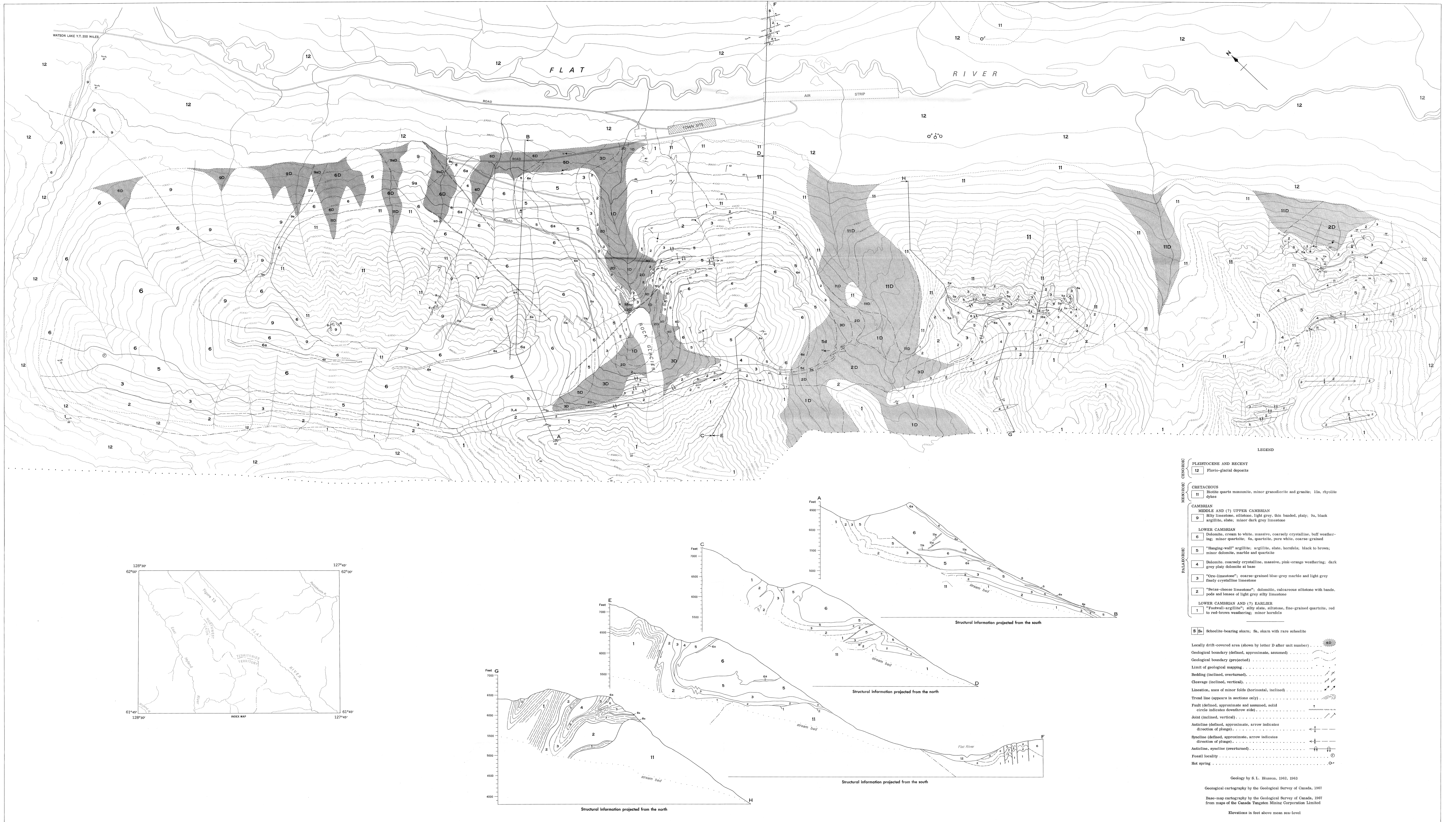
Figure 13. Geology in the vicinity of the Canada Tungsten mine, Yukon Territory and District of Mackenzie.
