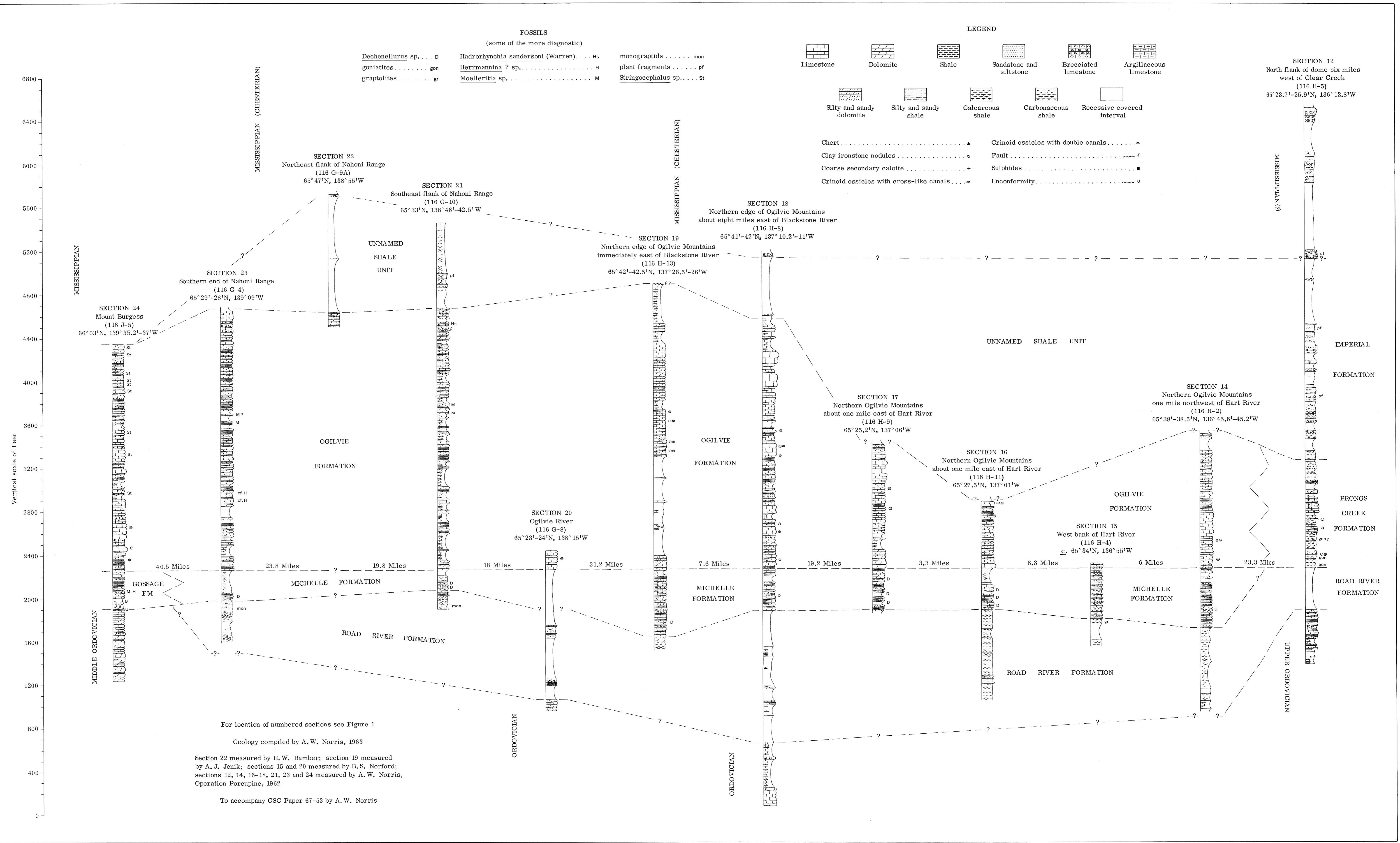
Figure 4. Stratigraphic sections of Devonian formations between Clear Creek anticline (section 12) and Mount Burgess (section 24).
