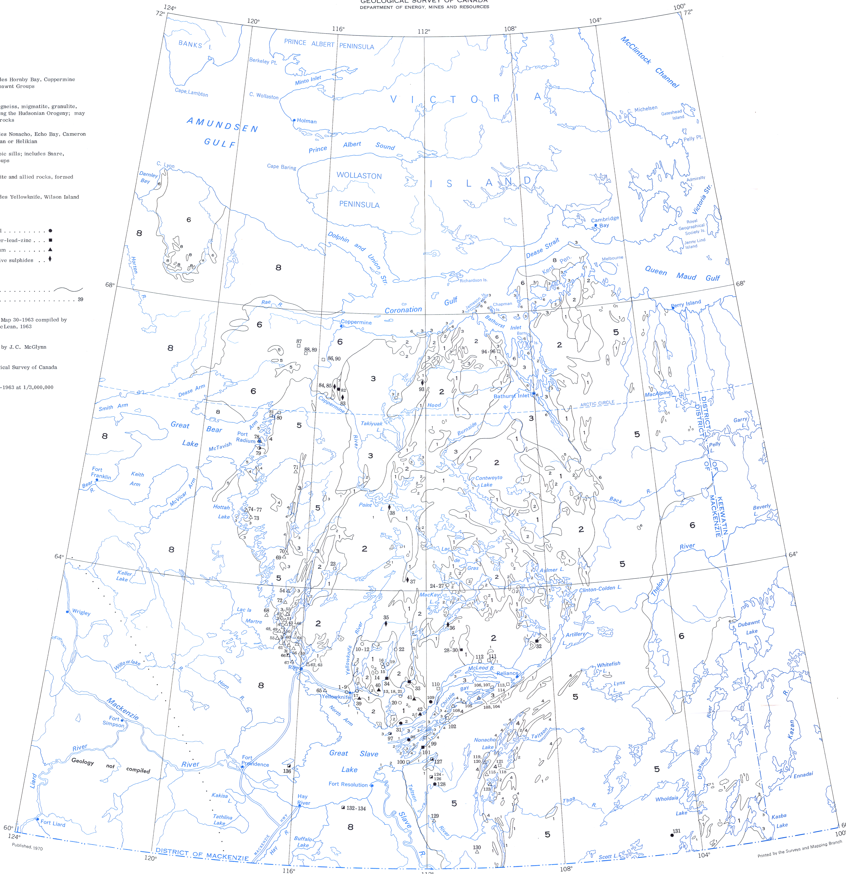
Figure 10. Simplified geology and index of properties, District of Mackenzie.
