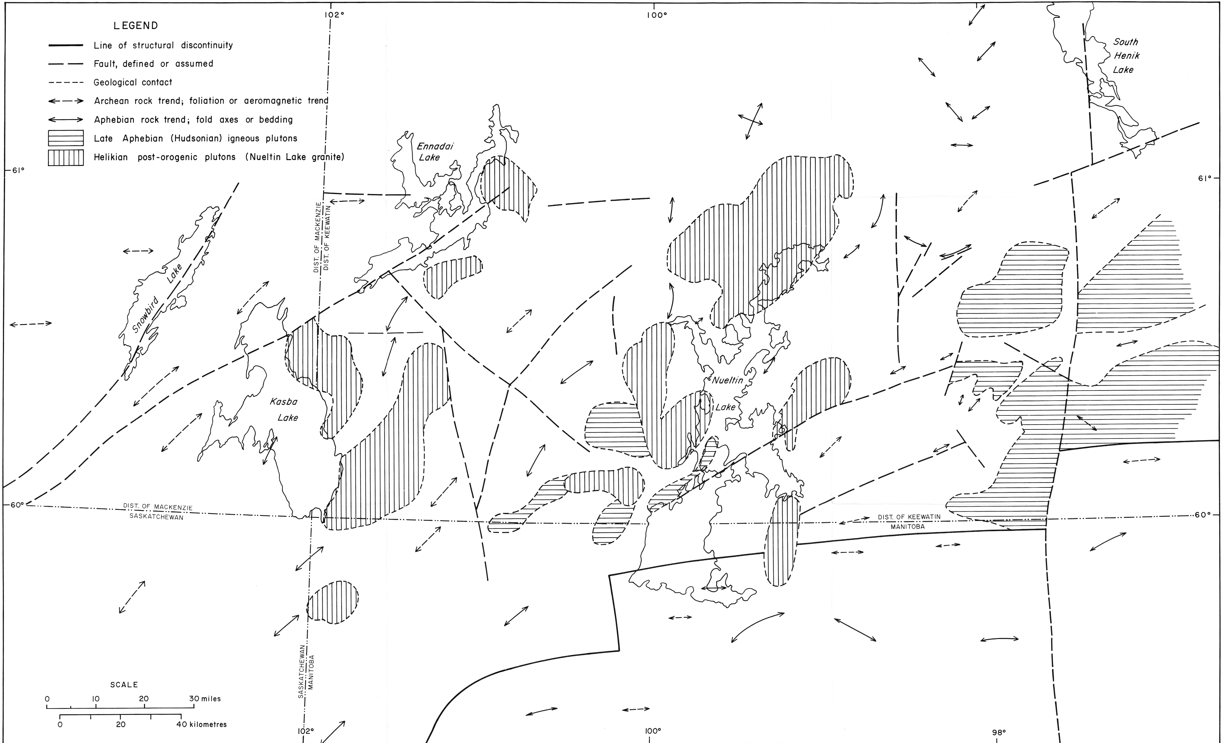
Figure 1. Regional pattern of tectonics and plutons in southwestern District of Keewatin and adjoining parts of Manitoba, Saskatchewan and District of Mackenzie
