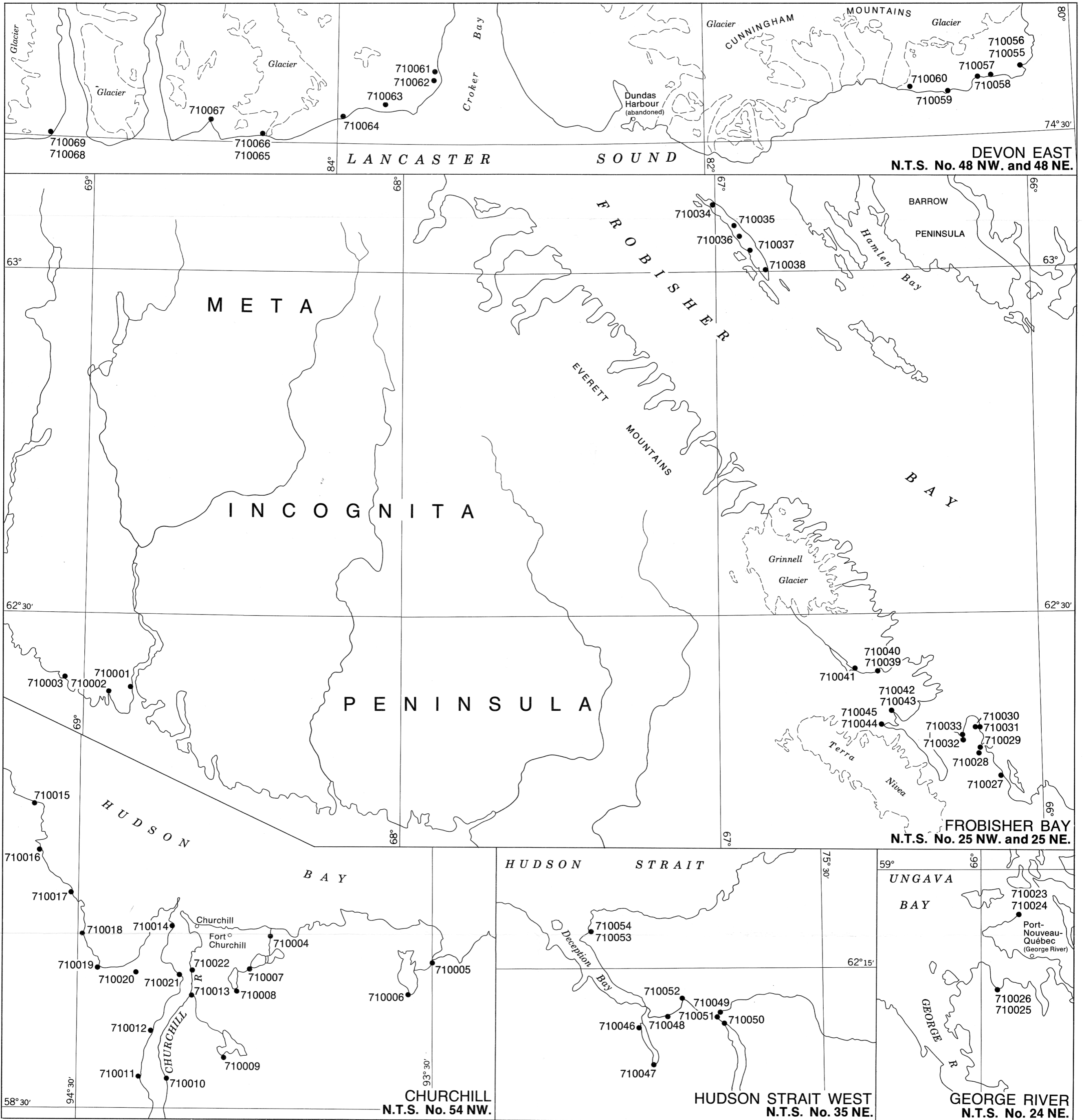
Figure 2. Geochemical sample locations on arctic coastal streams, Districts of Franklin and Keewatin
