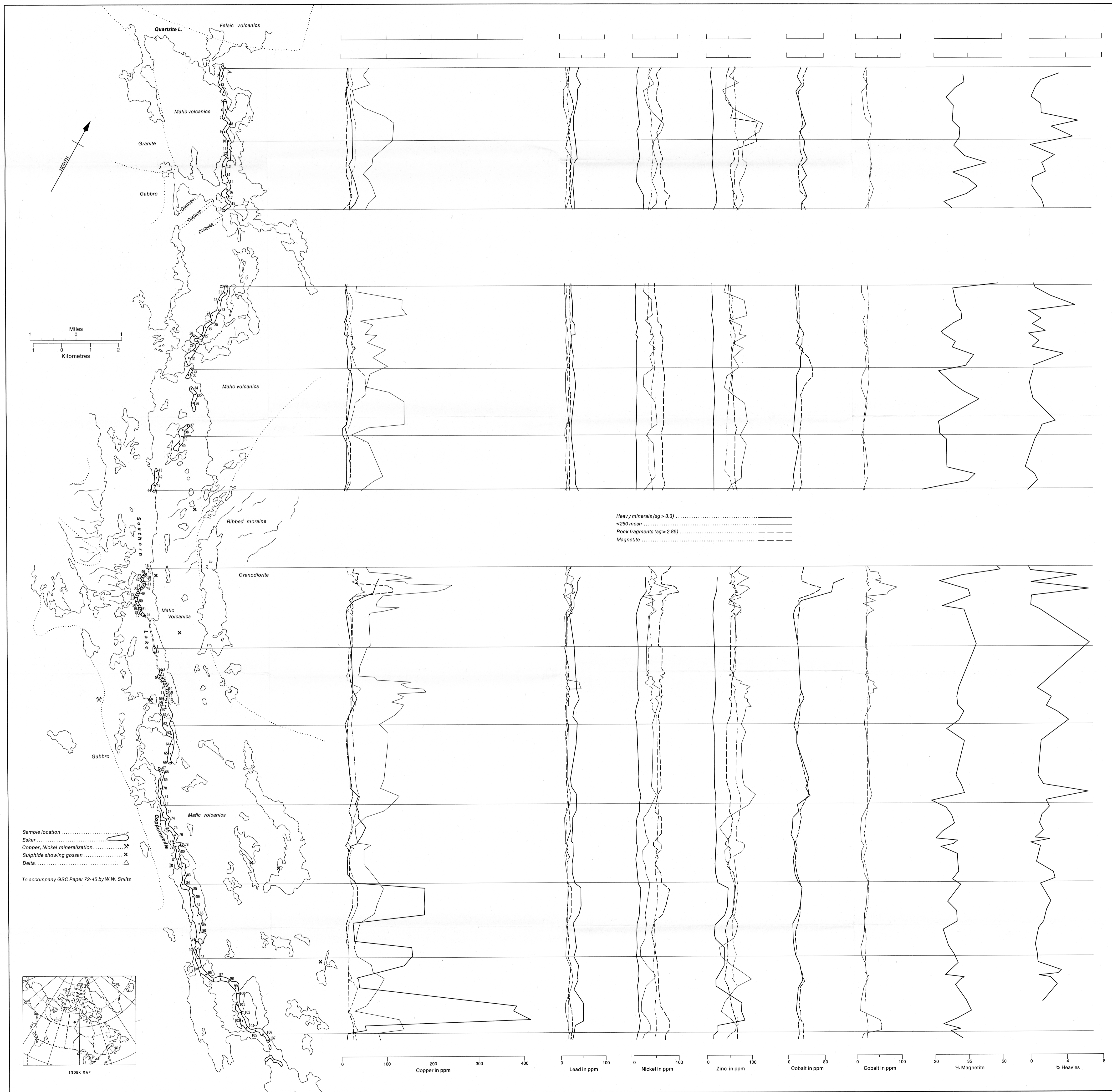
Figure 6. Trace-element variations in various fractions of the Copperneedle Esker, District of Keewatin.
