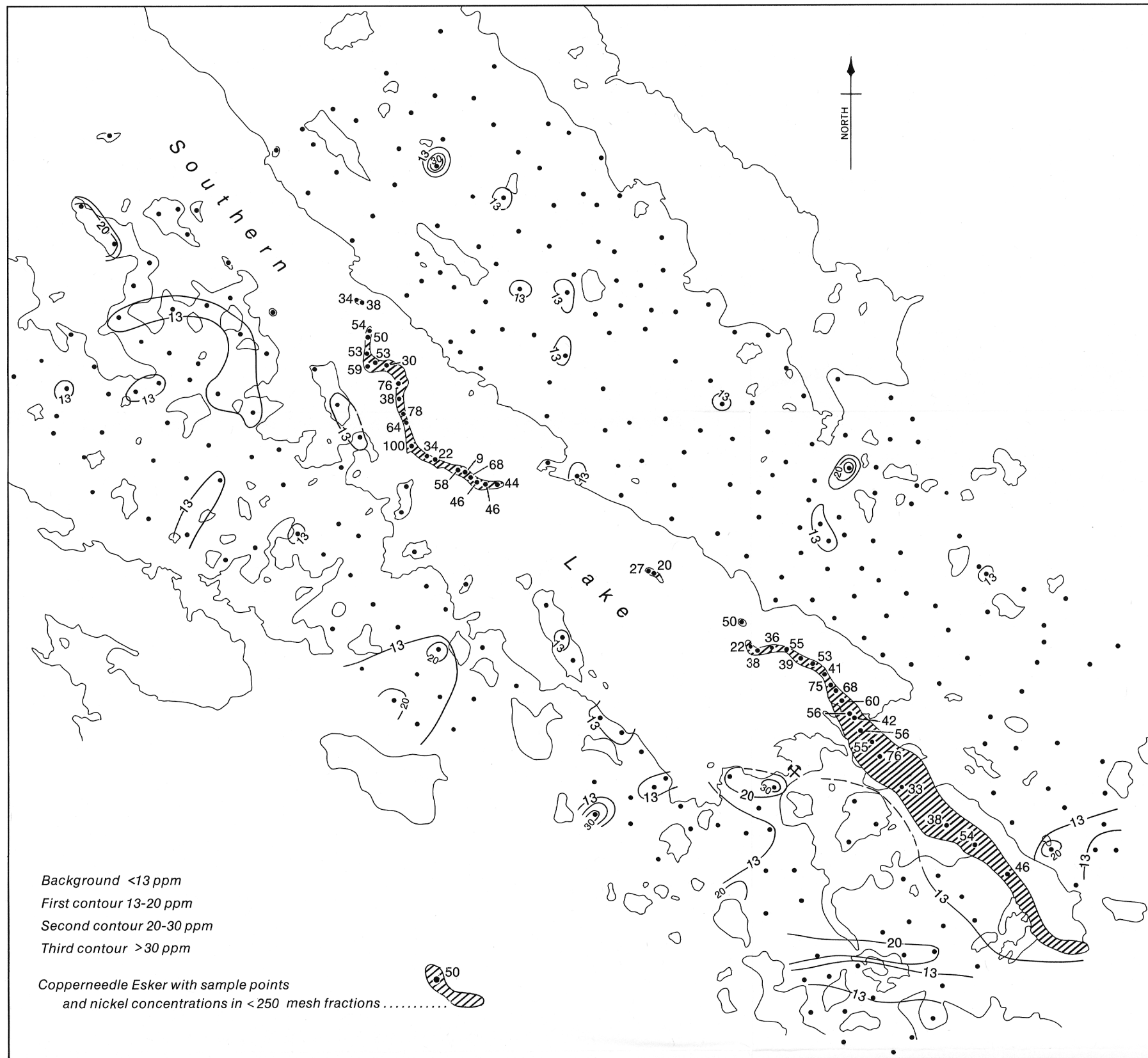
Nickel in -250 mesh (-64 μ) fraction of till
