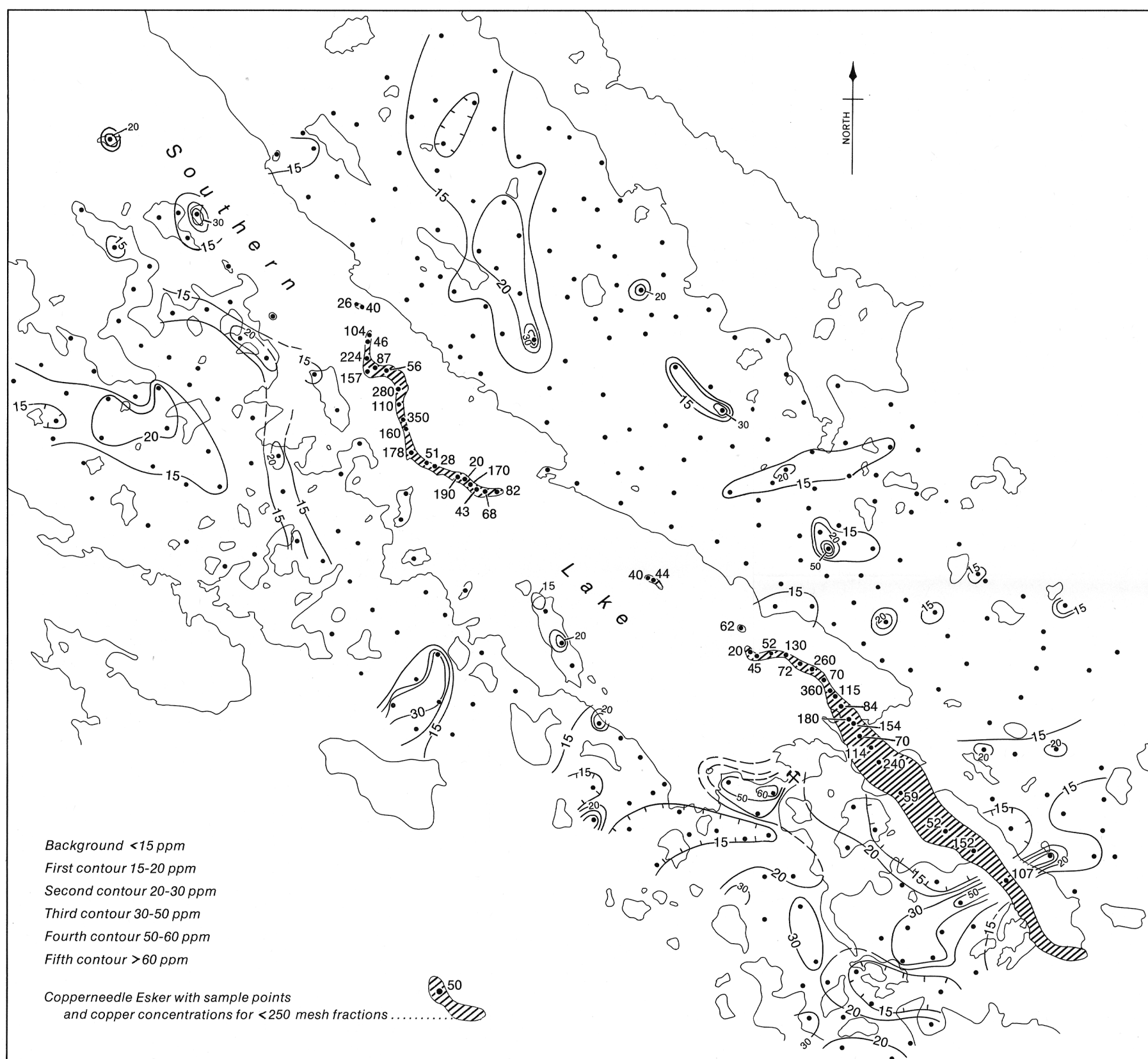
Copper in -250 mesh (-64 μ) fraction of till
