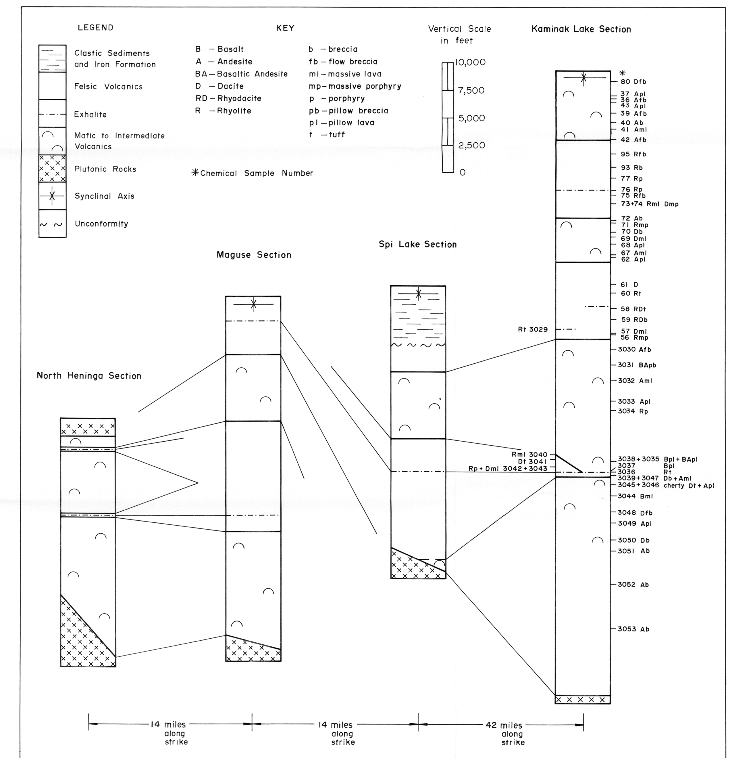
Figure 16. Stratigraphy of the Kaminak Group, Spi Lake area, District of Keewatin
