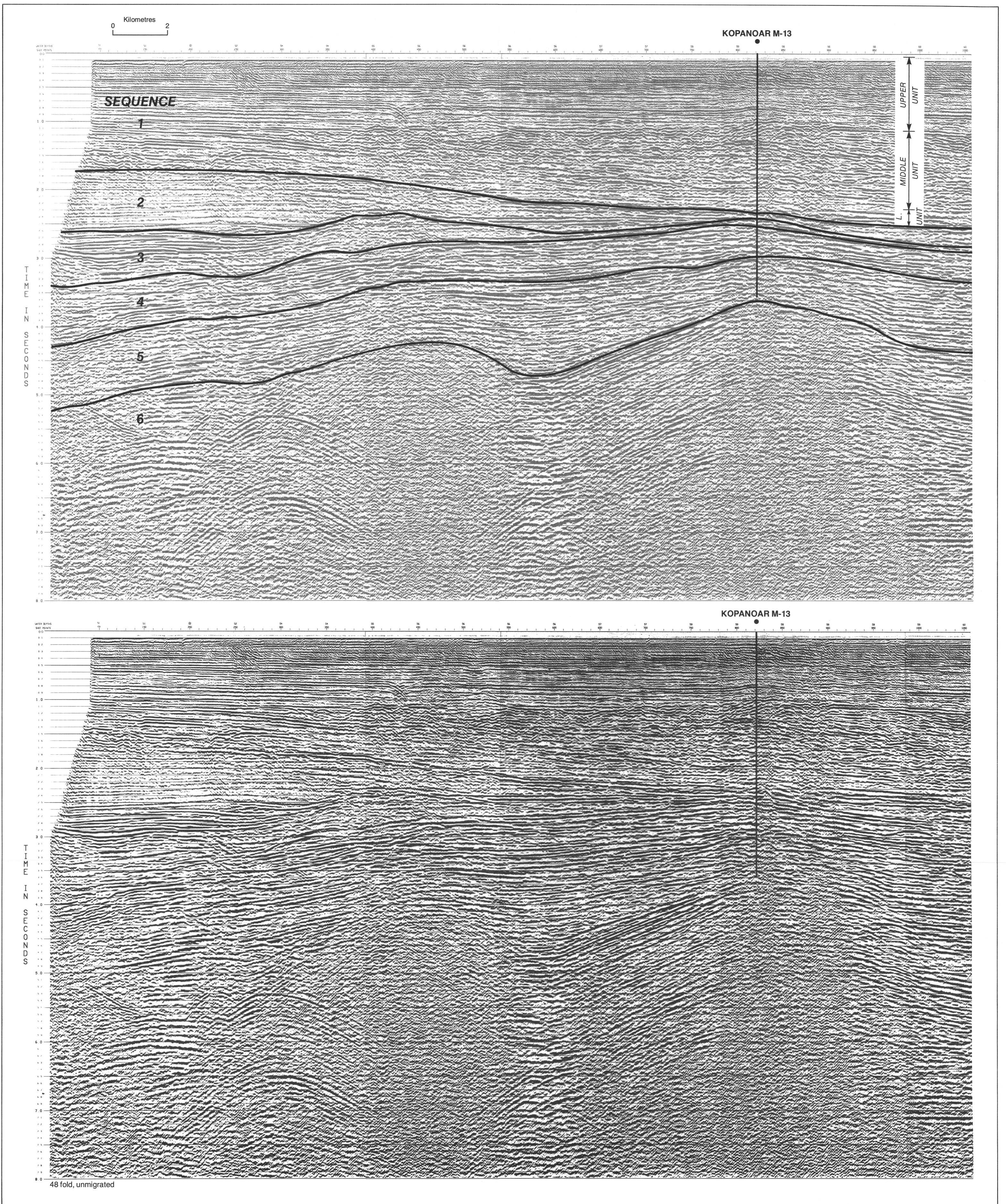
Figure 2. Reflection seismic profile through the Kopanoar M-13 well. Top profile is interpreted to show the sequence boundaries; bottom profile is uninterpreted. (Dome Petroleum is gratefully acknowledged for permission to publish the seismic data.)
