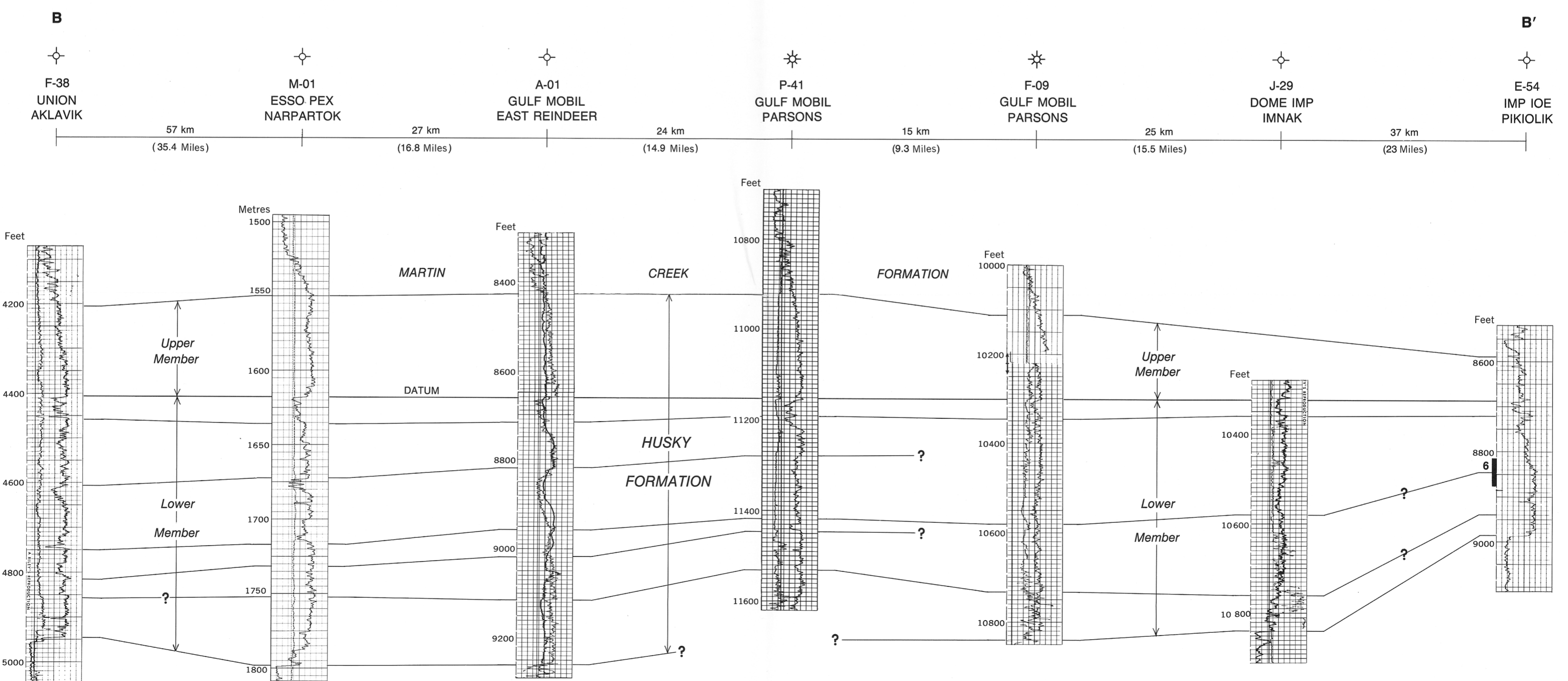
Figure 11. Cross section B-B' utilizing gamma ray logs
