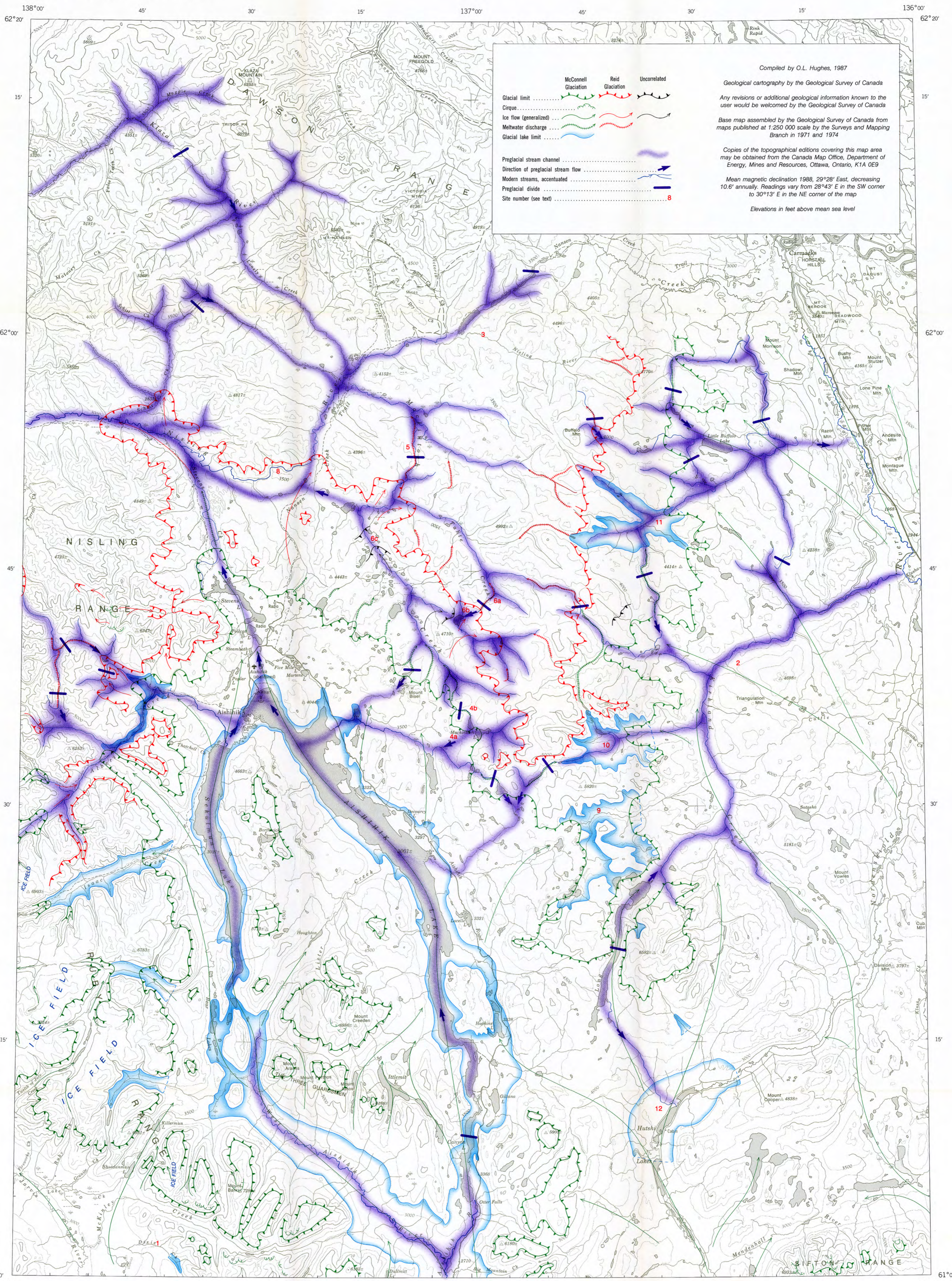
Figure 3. Glacial limits, ice flow patterns, glacial lakes, and glacially induced drainage changes, Aishihik Lake and Southern Carmacks map areas, Yukon Territory
