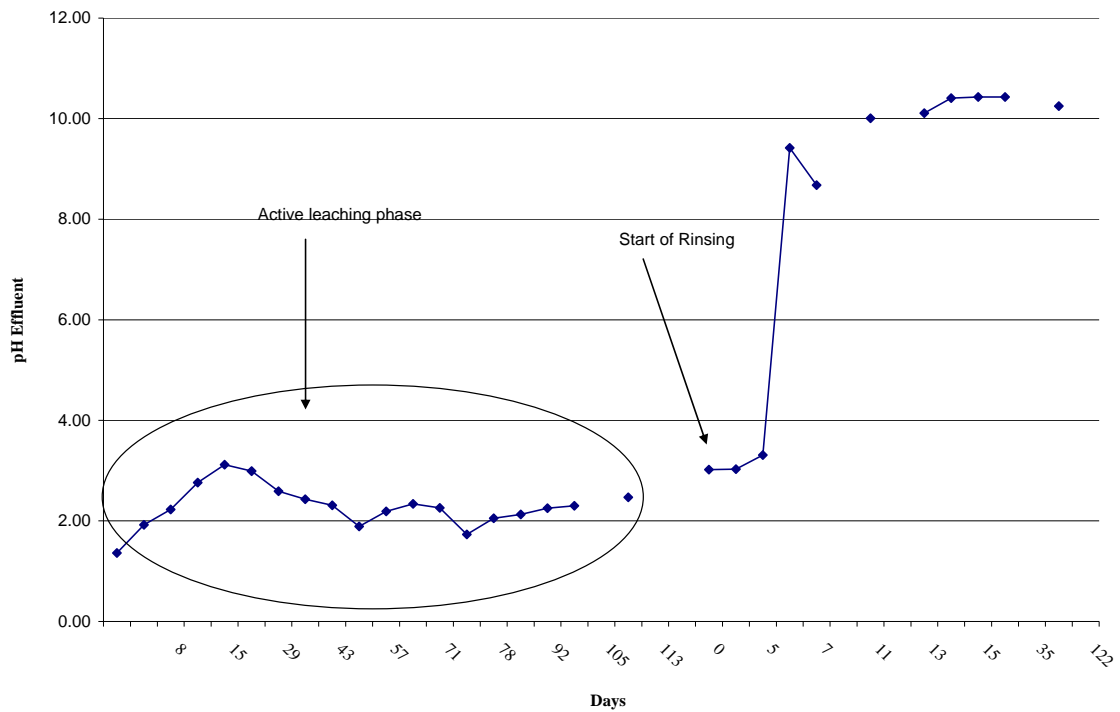
Figure 4 Carmacks Copper Column Detox Results Column 5 Parameter - pH
