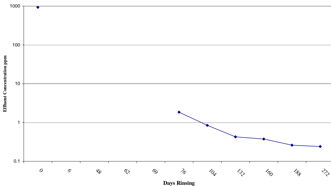
Figure 7 Carmacks Copper Column Detox Results Column 9 Parameter - Copper
