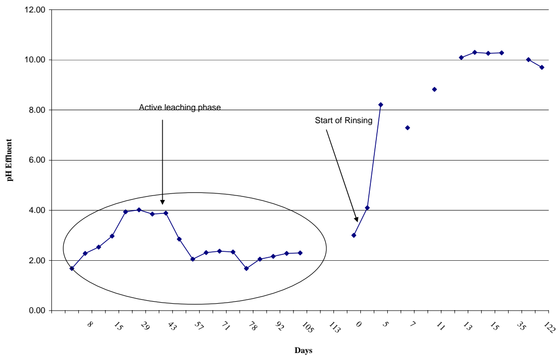
Figure 5 Carmacks Copper Column Detox Results Column 8 Parameter - pH
